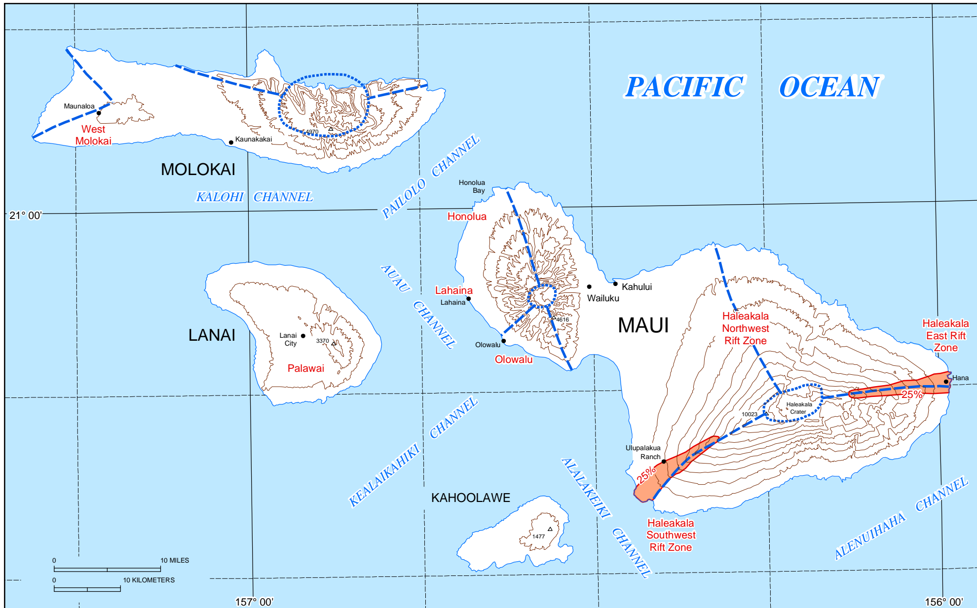
Figure 4: Geothermal resource areas of Maui County
