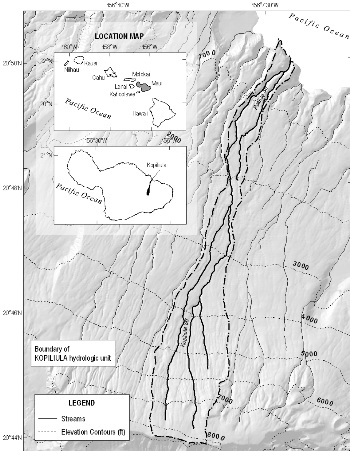
Figure 1-4. Elevation range and the location of Kopiliula hydrologic unit. (Source: State of Hawaii, Office of Planning, 1983; USGS, 2001b).
