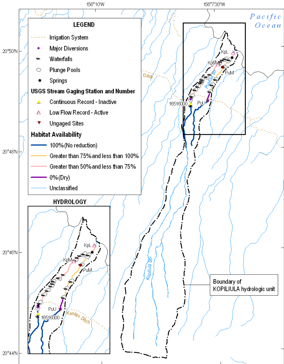
Figure 4-3. Estimated habitat availability in Kopiliula hydrologic unit (Source: Gingerich and Wolff, 2005; USGS, 2001b).
