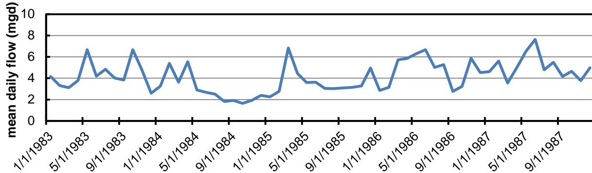
Figure 13-1 Mean daily flow (in million gallons per day, mgd) in Ukumehame Ditch diverted from Ukumehame Stream from 1983 to 1988 as reported in the registration index by Pioneer Mill.
