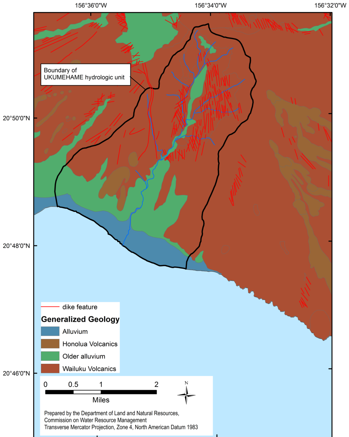
Figure 2-2. Generalized geology of the Ukumehame hydrologic unit. (Source: Sherrod et al., 2007)
