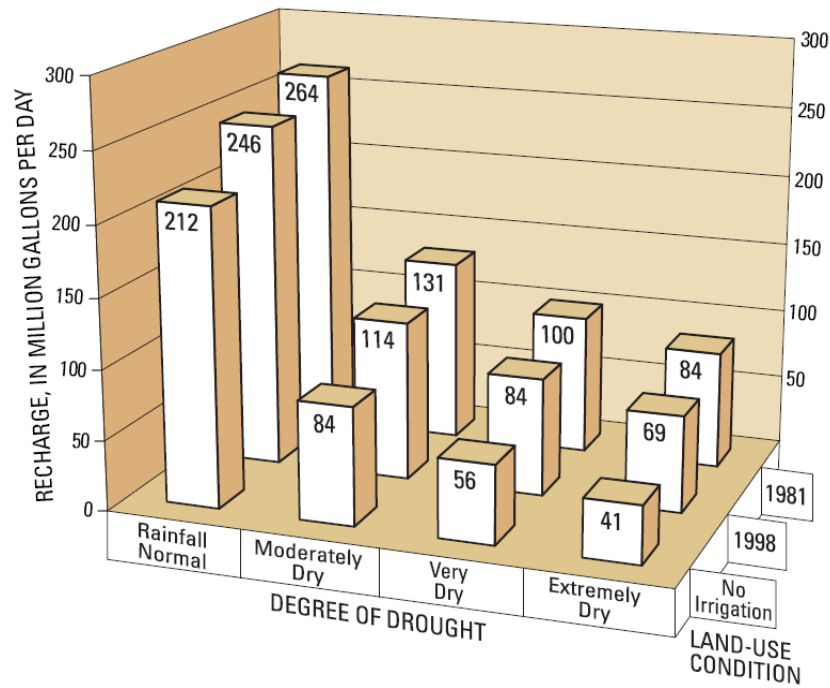
Figure 13-4. Summary of estimated recharge, in million gallons per day, for various land-use and rainfall conditions in the Lihue Basin, Kauai, Hawaii. (Source: Izuka et al., 2005)
