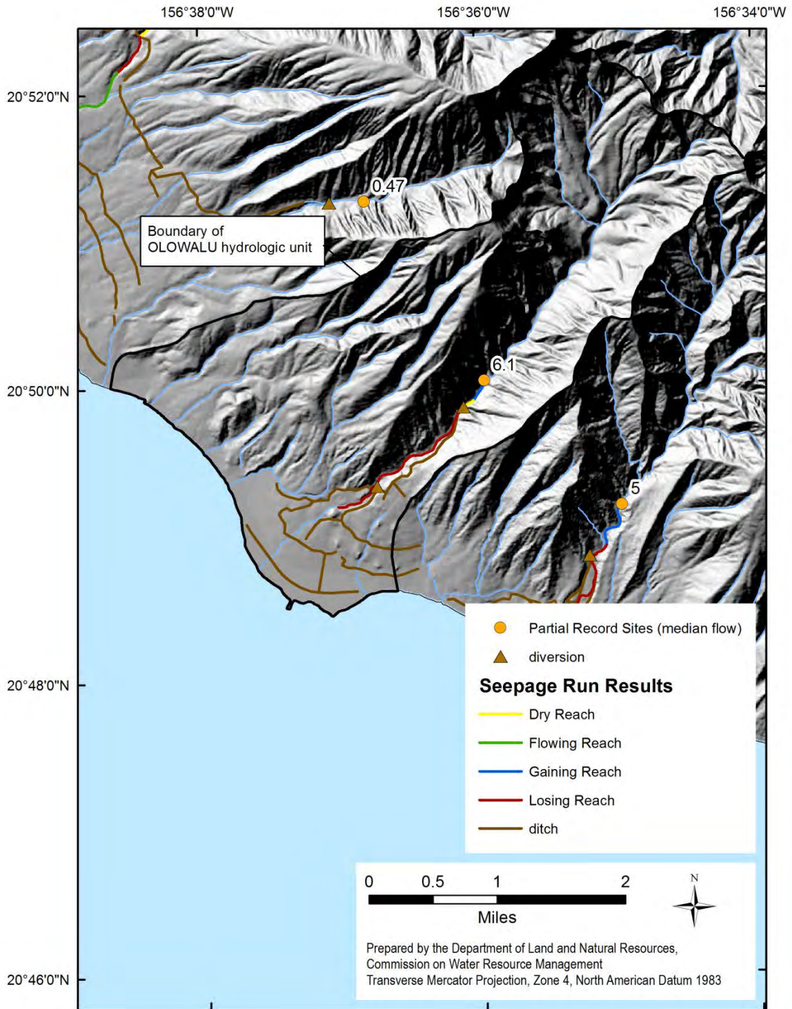
Figure 3-4. Seepage run results and median flow from partial record gaging stations of the Olowalu hydrologic unit (Source: State of Hawaii, Commission on Water Resource Management, 2015a; Cheng, 2014).
