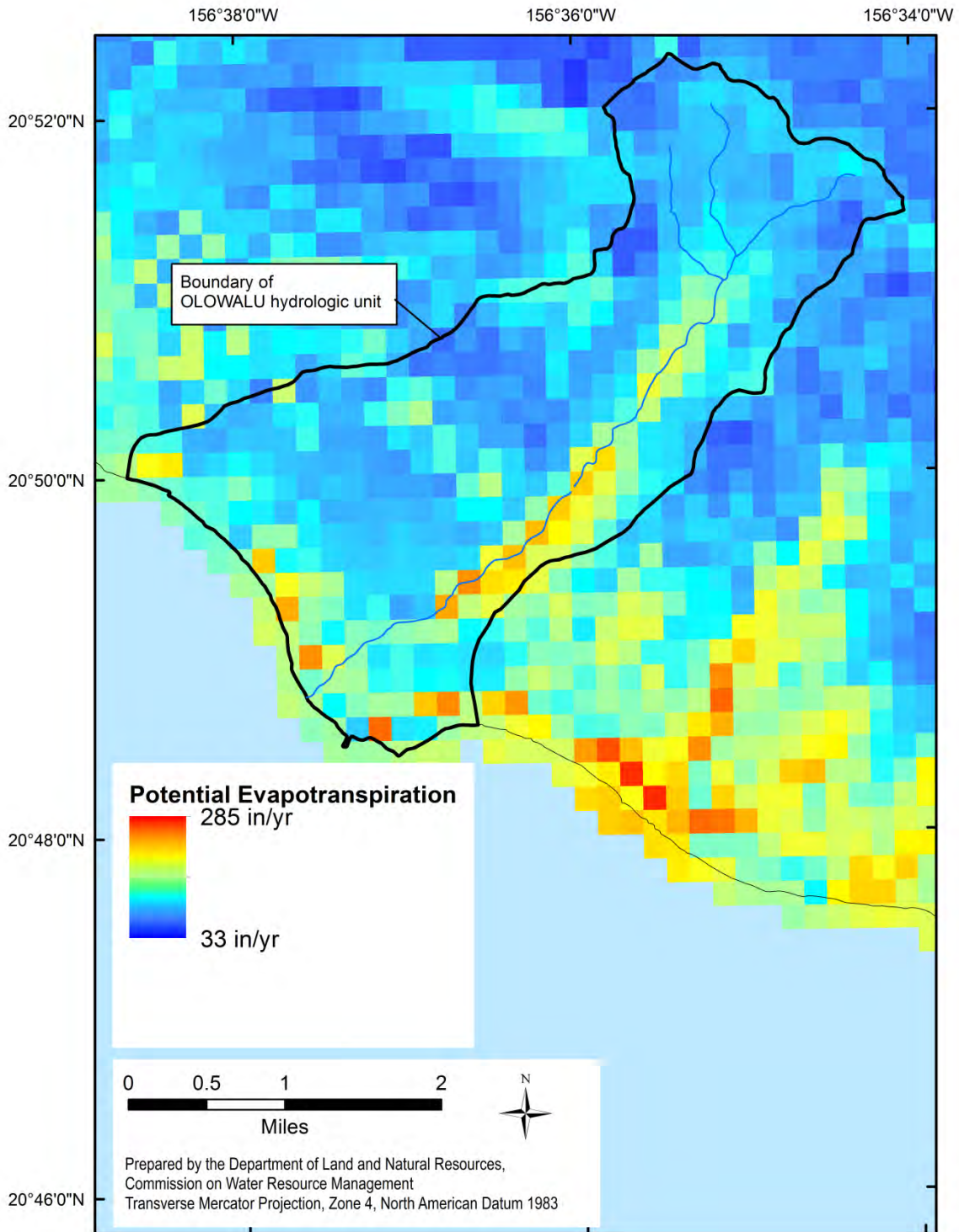
Figure 2-6. Mean annual potential evapotranspiration (Penman-Monteith method) of the Olowalu hydrologic unit. (Source: Giambelluca et al., 2014)
