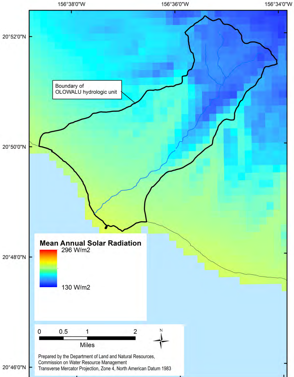
Figure 2-5. Mean annual solar radiation of the Olowalu hydrologic unit. (Source: State of Hawaii, Office of Planning, 2015c)
