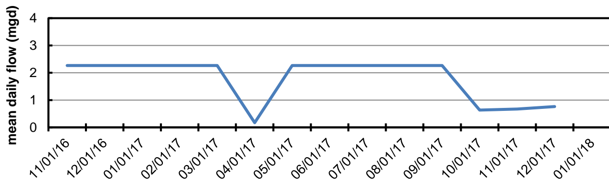
Figure 13-8. Mean daily flow (million gallons per day, mgd) diverted by Olowalu Water Co. from Olowalu Stream at the lower diversion into Olowalu Ditch calculated from monthly data for 2016 and 2017. (Source: CWRM database)
