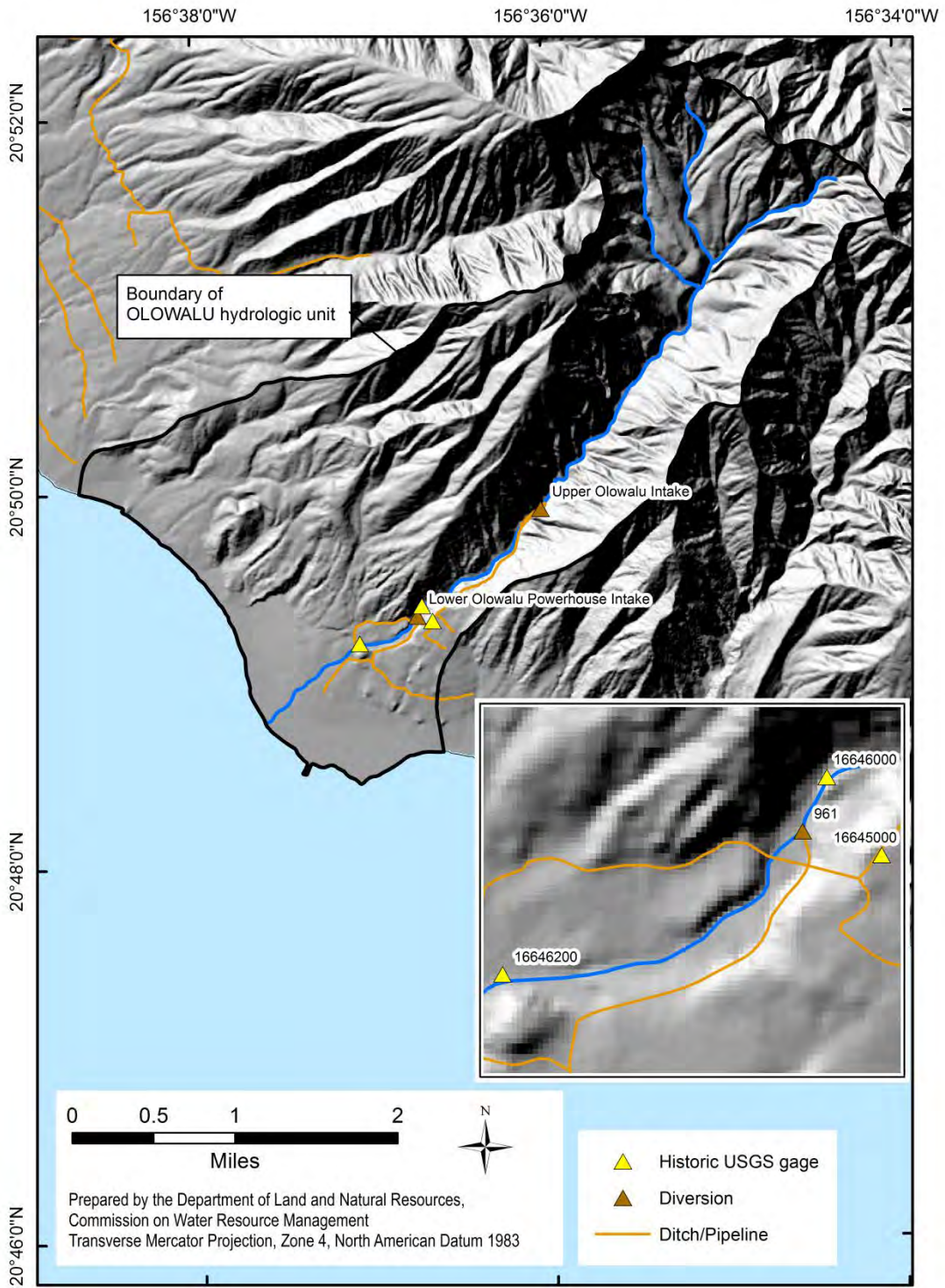
Figure 3-3. Ditches, diversions and USGS gaging stations in the Olowalu hydrologic unit (Source: State of Hawaii, Commission on Water Resource Management, 2015a).
