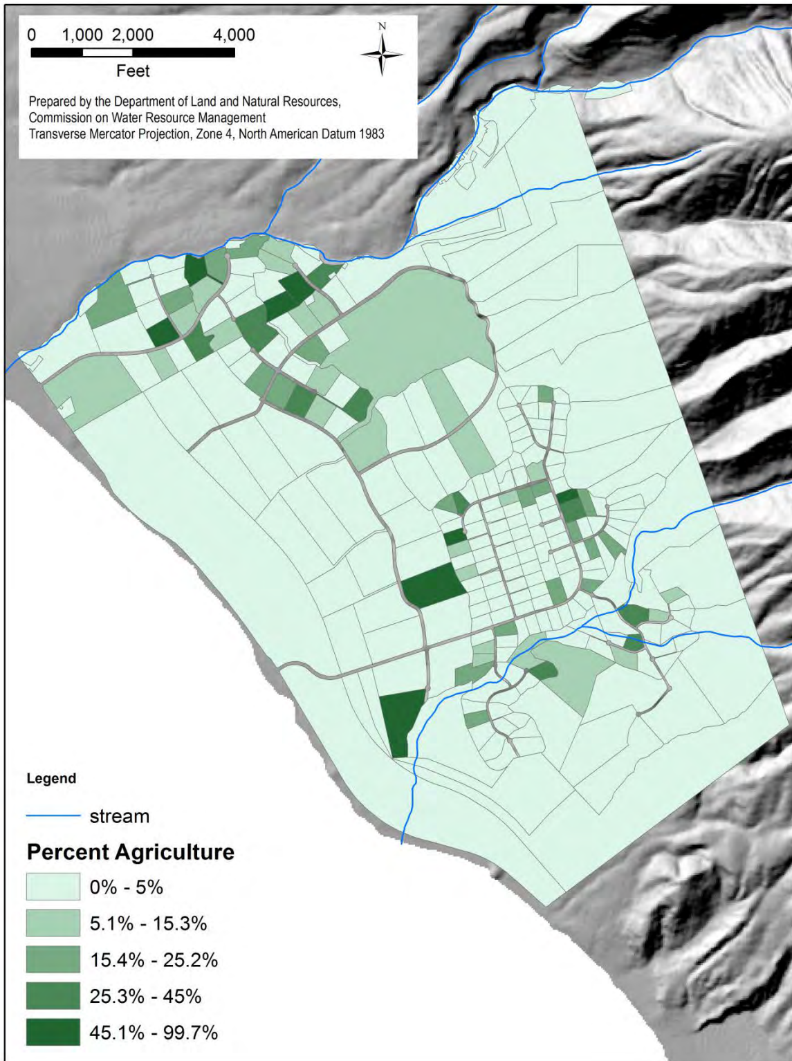
Figure 13-9 Percent of each TMK in the Launiupoko Irrigation Company service area in agriculture as determined using remote sensing.
