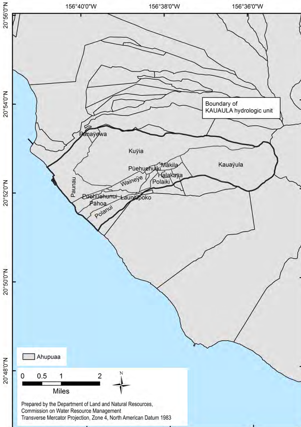
Figure 12-1. Traditional ahupuaa boundaries in the vicinity of Kaua'ula hydrologic unit. (Source: State of Hawaii, Office of Planning, 2015)
