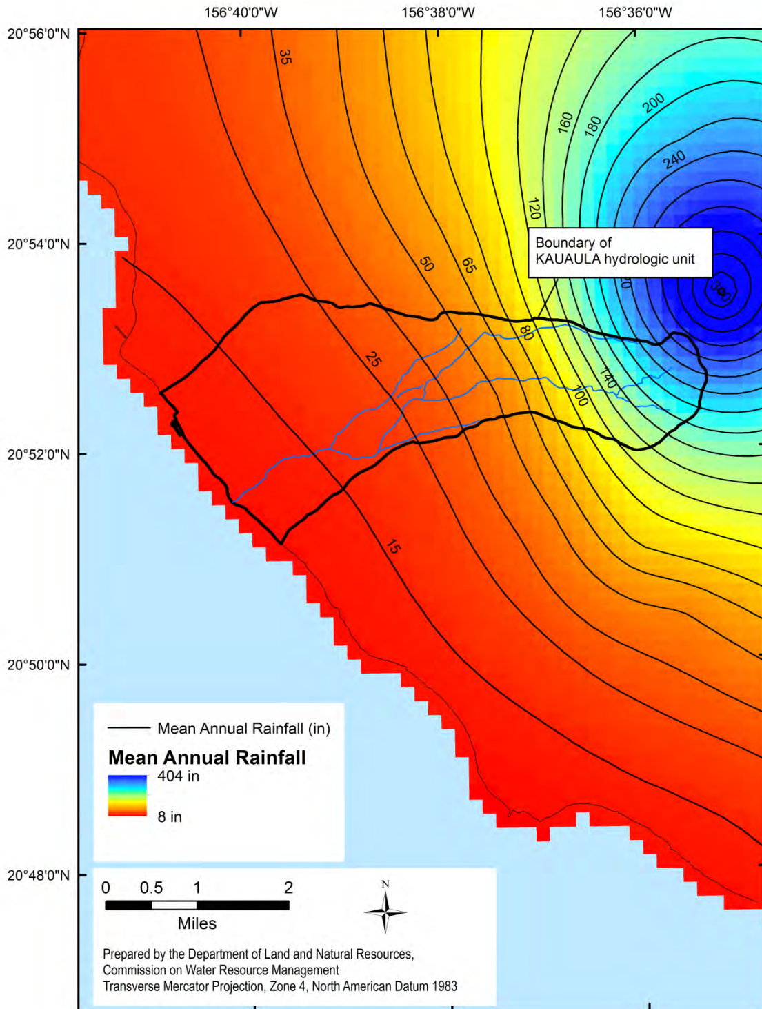
Figure 2-4. Mean annual rainfall of the Kauaula hydrologic unit. (Source: Giambelluca et al., 2013)
