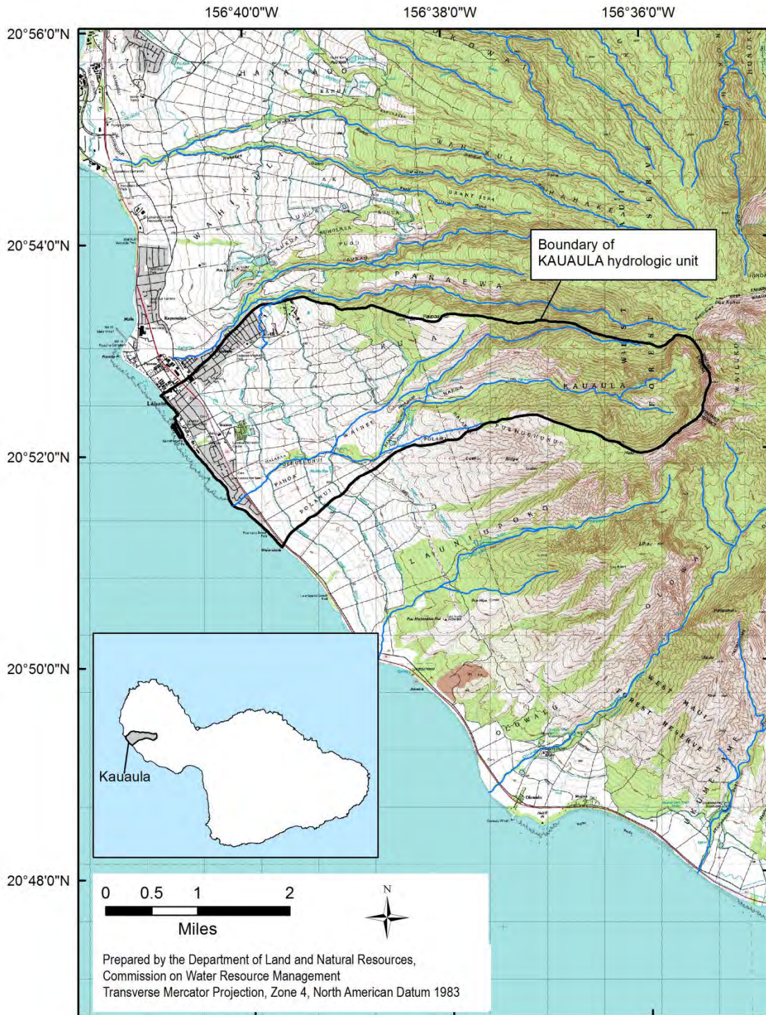
Figure 1-5. USGS topographic map of the Kauaula hydrologic unit. (Source: State of Hawaii, Planning Department, 2004)
