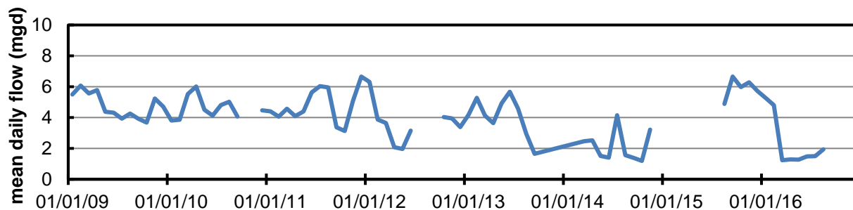
Figure 13-8. Mean daily flow (million gallons per day, mgd) diverted by Launiupoko Irrigation Co. from Kauaula Stream to Kauaula Ditch calculated from monthly data from 2009-2016. (Source: Lea Tamayose, West Maui Land Co.)
