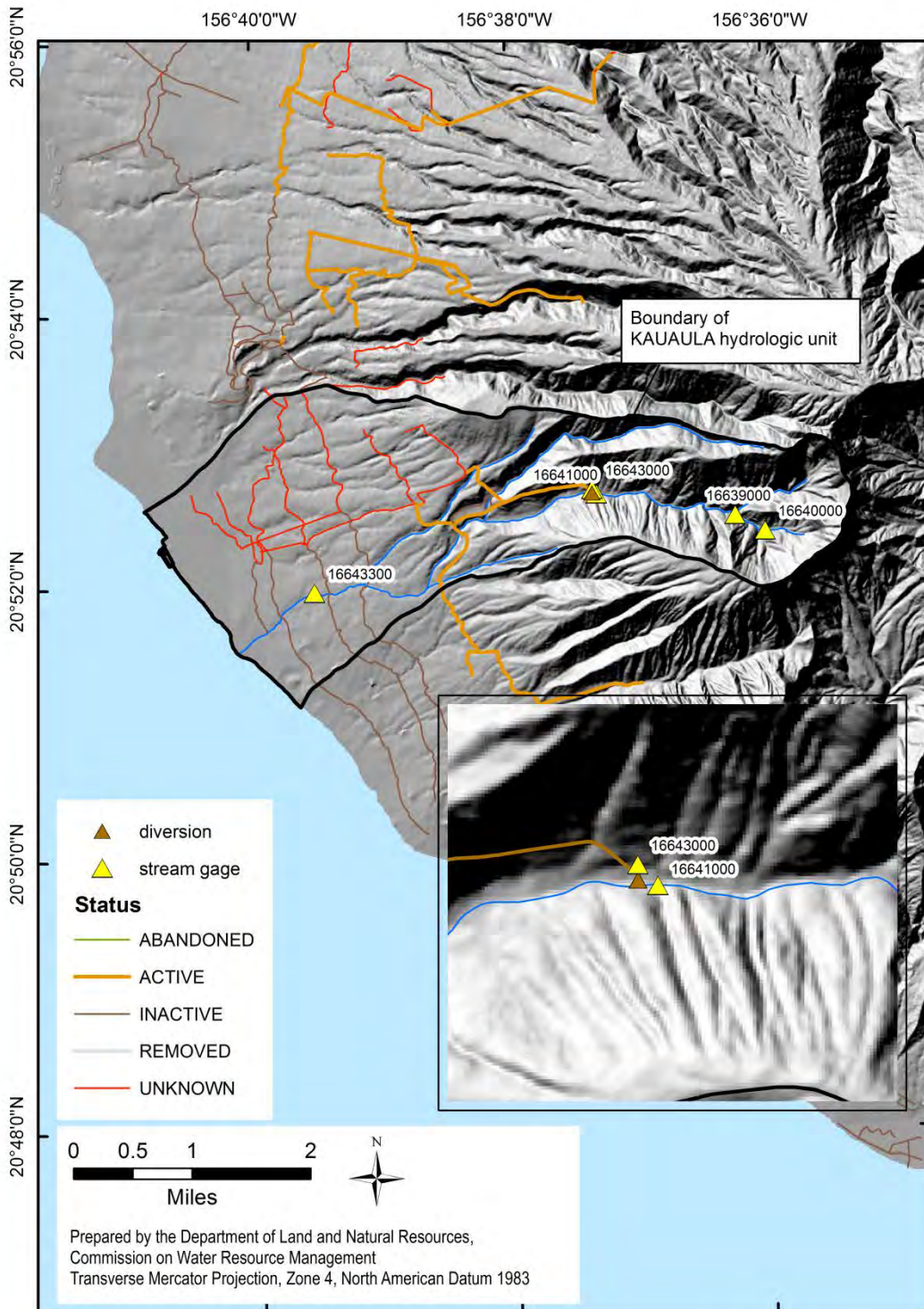
Figure 3-2. Ditches, diversions and USGS gaging stations in the Kauaula hydrologic unit (Source: State of Hawaii, Commission on Water Resource Management, 2015a).
