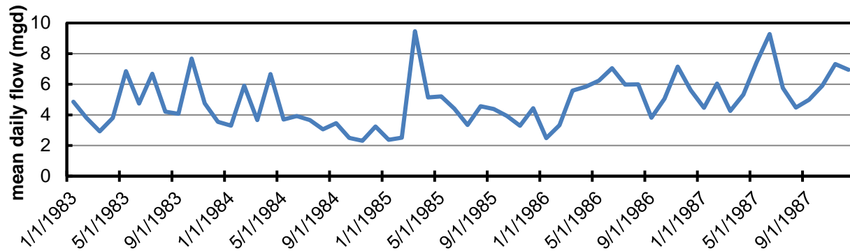
Figure 13-7. Mean daily flow (million gallons per day, mgd) diverted by Pioneer Mill from Kauaula Stream into Kauaula Ditch calculated from monthly data from 1983-1987. (Source: Pioneer Mill Co Registration, DIV.956.6)
