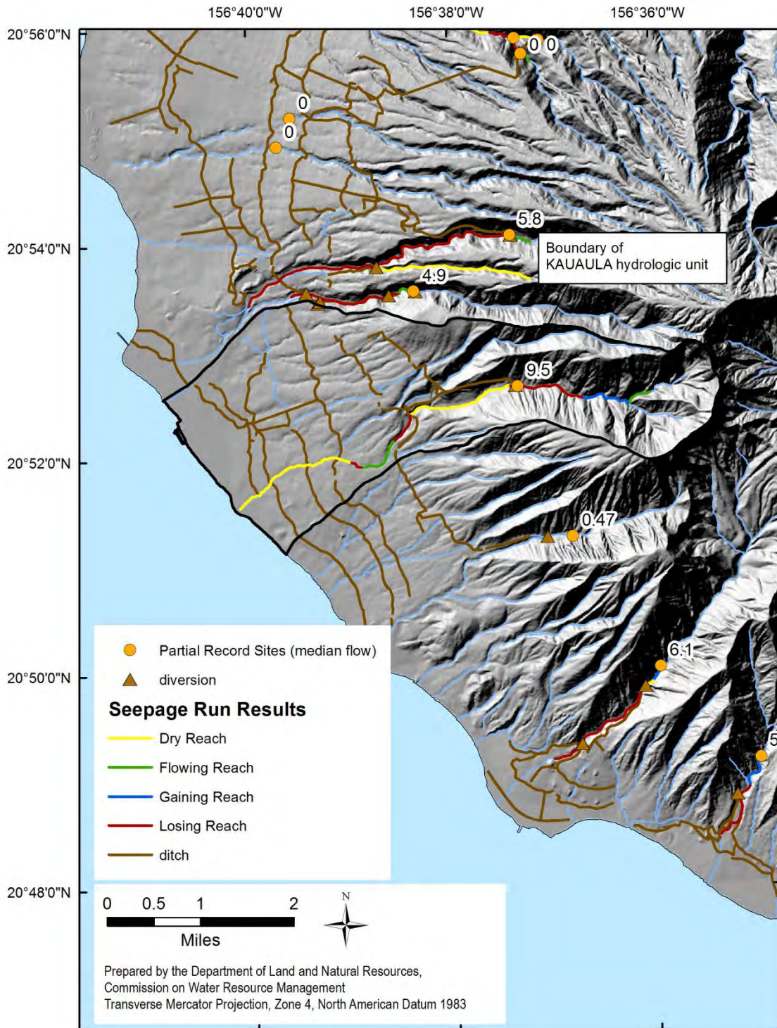
Figure 3-3. Seepage run results from 2012 and median flow from partial record gaging stations of the Kauaula hydrologic unit (Source: State of Hawaii, Commission on Water Resource Management, 2015a; Cheng, 2014).
