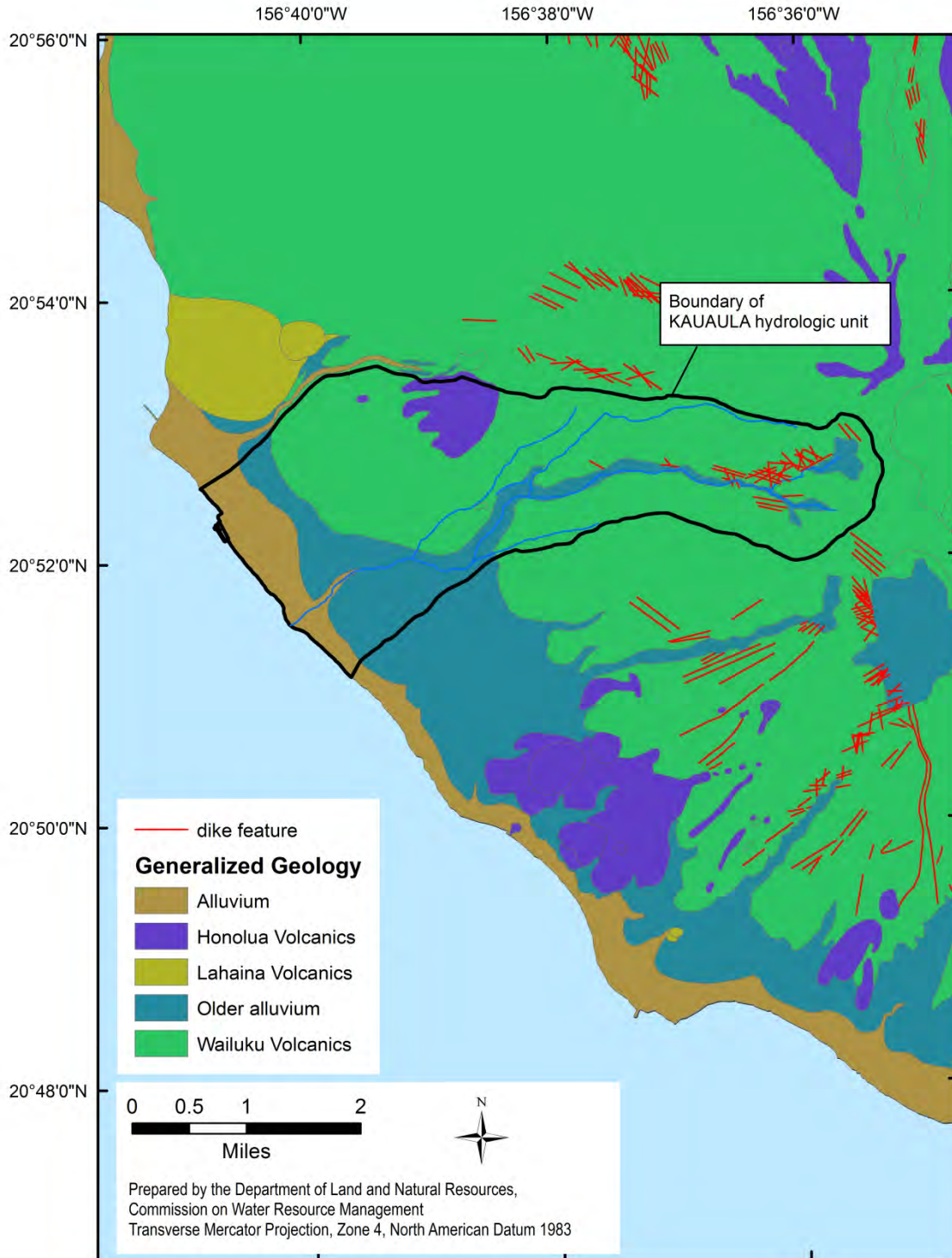
Figure 2-2. Generalized geology of the Kauaula hydrologic unit. (Source: Sherrod et al., 2007)
