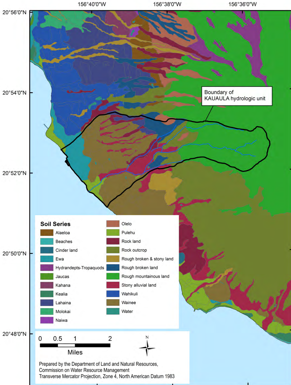
Figure 2-3. Soil classification in the Kauaula hydrologic unit. (Source: State of Hawaii, Office of Planning, 2015m)
