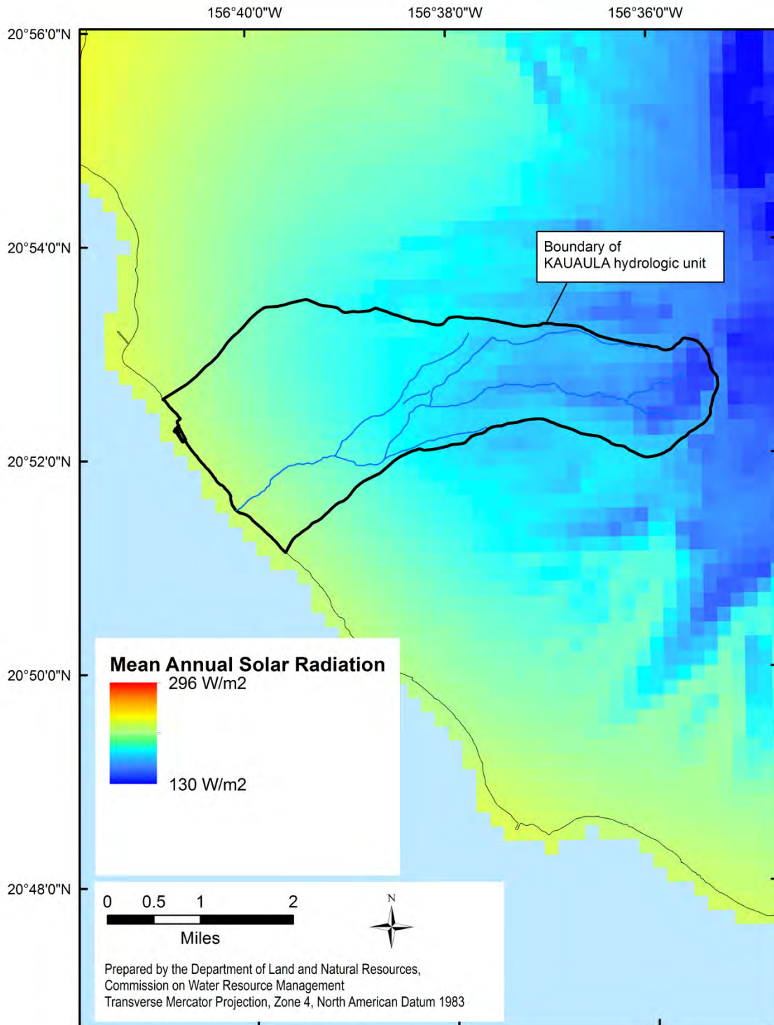
Figure 2-5. Mean annual solar radiation of the Kauaula hydrologic unit. (Source: State of Hawaii, Office of Planning, 2015c)
