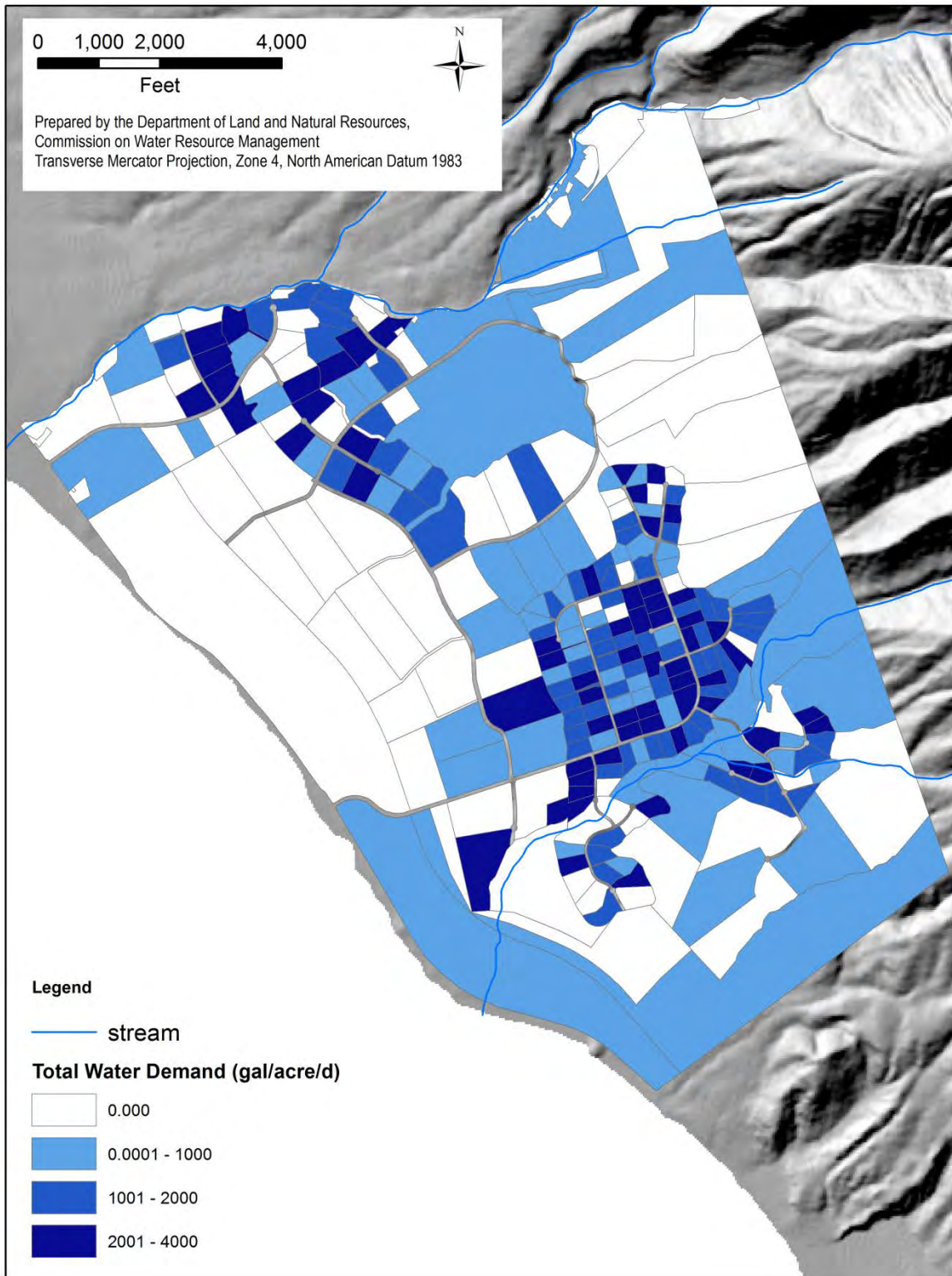
Figure 13-11. Estimated water demand of each TMK in the Launiupoko Irrigation Company service area based on land cover (agriculture or landscaping) using remote sensing and modeled water demand for that land cover.
