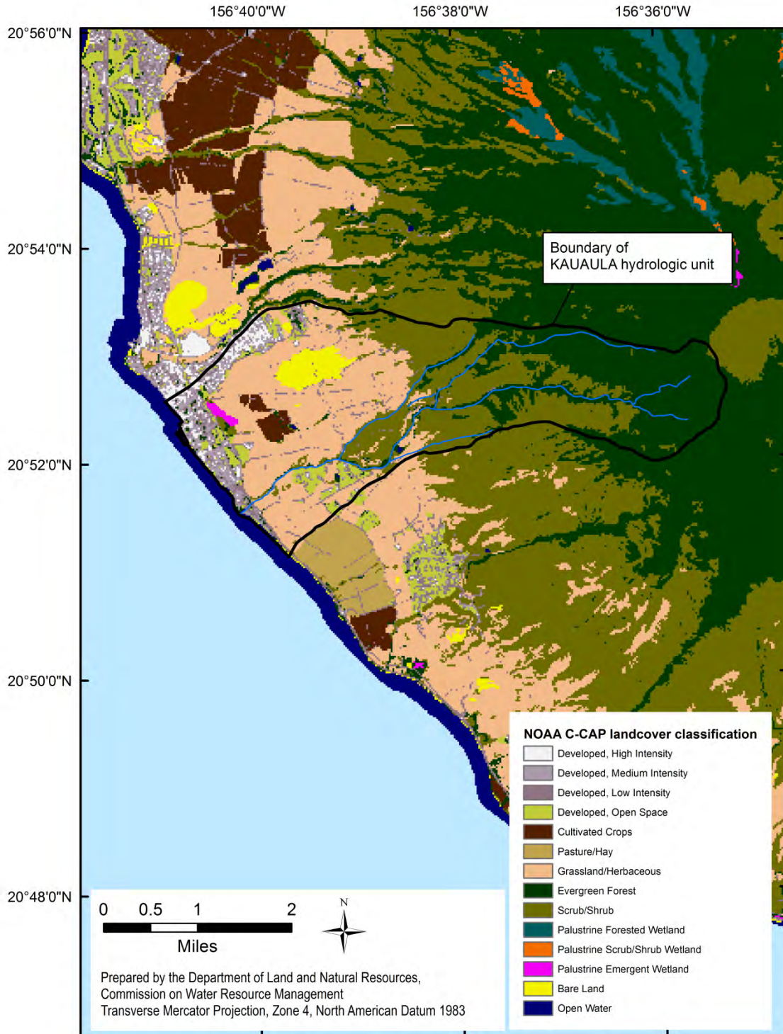
Figure 2-8. C-CAP land cover of the Kauaula hydrologic unit. (Source: State of Hawaii, Office of Planning, 2015k).
