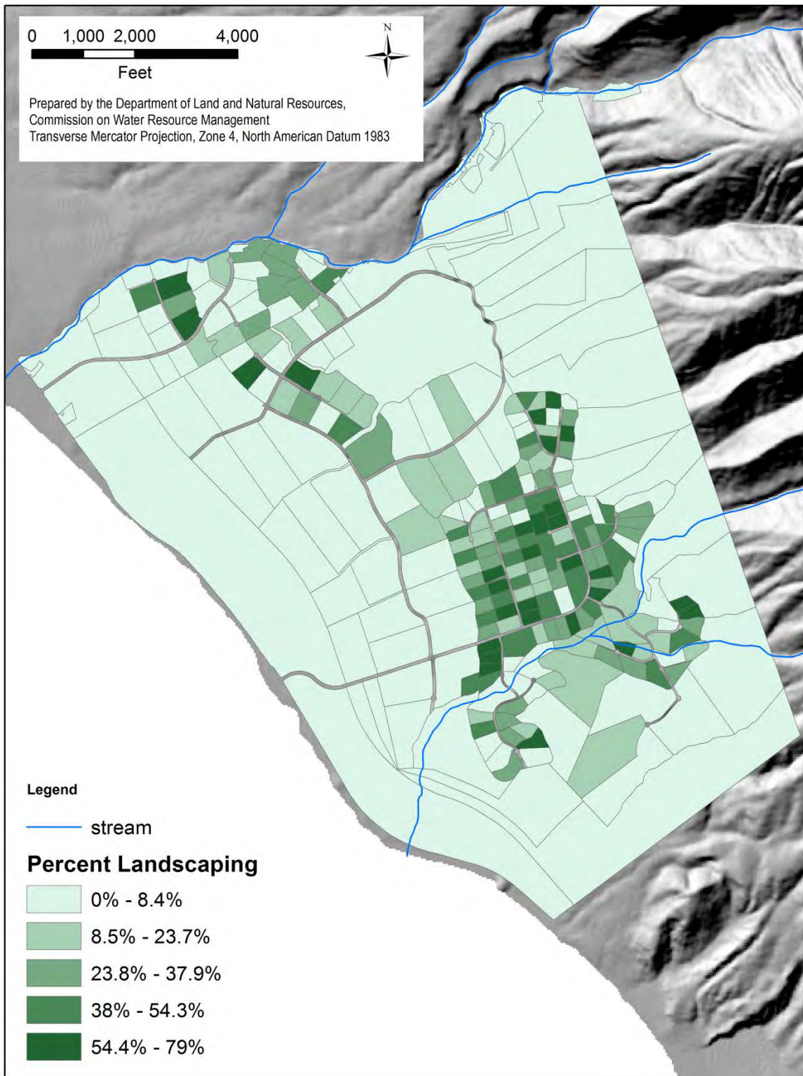
Figure 13-10. Percent of each TMK in the Launiupoko Irrigation Company service area in landscaping as determined using remote sensing.
