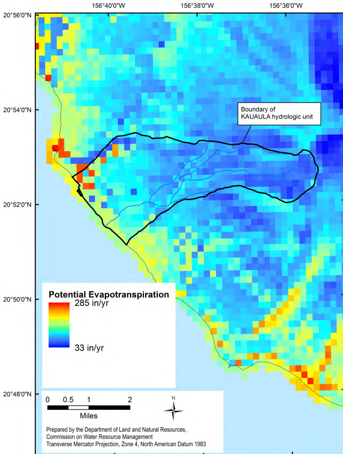
Figure 2-6. Mean annual potential evapotranspiration (Penman-Monteith method) of the Kauaula hydrologic unit. (Source: Giambelluca et al., 2014)
