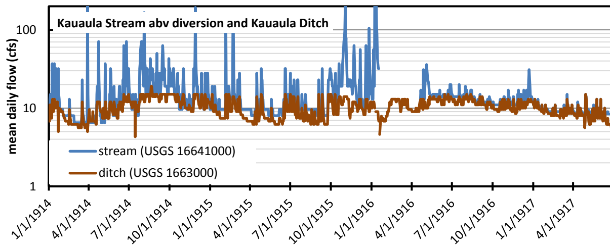
Figure 13-6. Mean daily flow (cubic feet per second, cfs) for Kauaula Stream and Kauaula Ditch based on USGS gaging records from January 1, 1914 to June 30, 1917.
