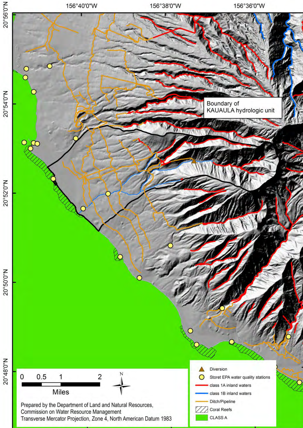
Figure 10-1. Water quality standards and monitoring locations for the Kauaula hydrologic unit. (Source: State of Hawaii, Office of Planning, 2015e; 2008). The classifications are general in nature and should be used in conjunction with Hawaii Administrative Rules, Chapter 11-54, Water Quality Standards.
