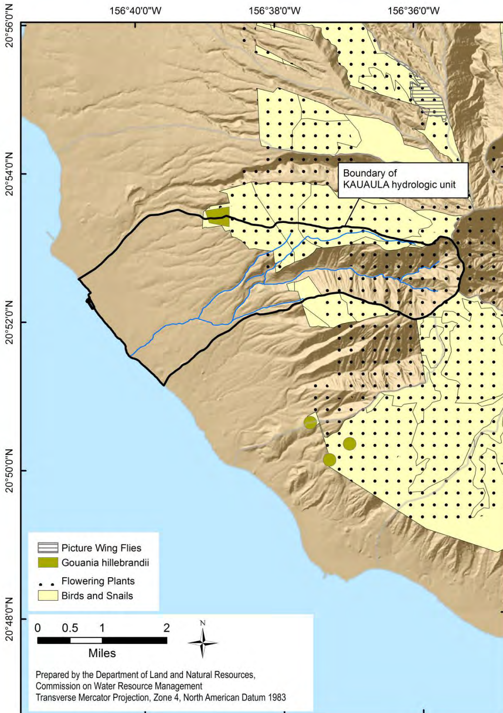
Figure 6-3. Distribution of critical habitat for particular endangered species including flies, flowering plants, birds and snails in the Kauaula hydrologic unit. (Source: Scott et al., 1986; State of Hawaii, Office of Planning, 1996; 2004b)
