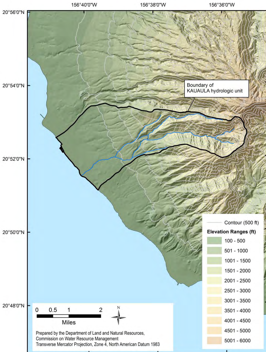
Figure 1-4. Elevation range of the Kauaula hydrologic unit. (Source: State of Hawaii, Office of Planning, 2004e; U.S. Geological Survey, 2001)
