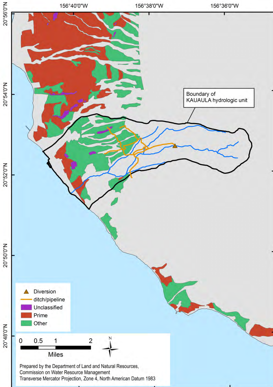
Figure 13-4. Agricultural land use for the Kauaula hydrologic unit based on the Agricultural Lands of Importance for the State of Hawaii (ALISH) classification systems. (Source: State of Hawaii, Office of Planning, 2015g)
