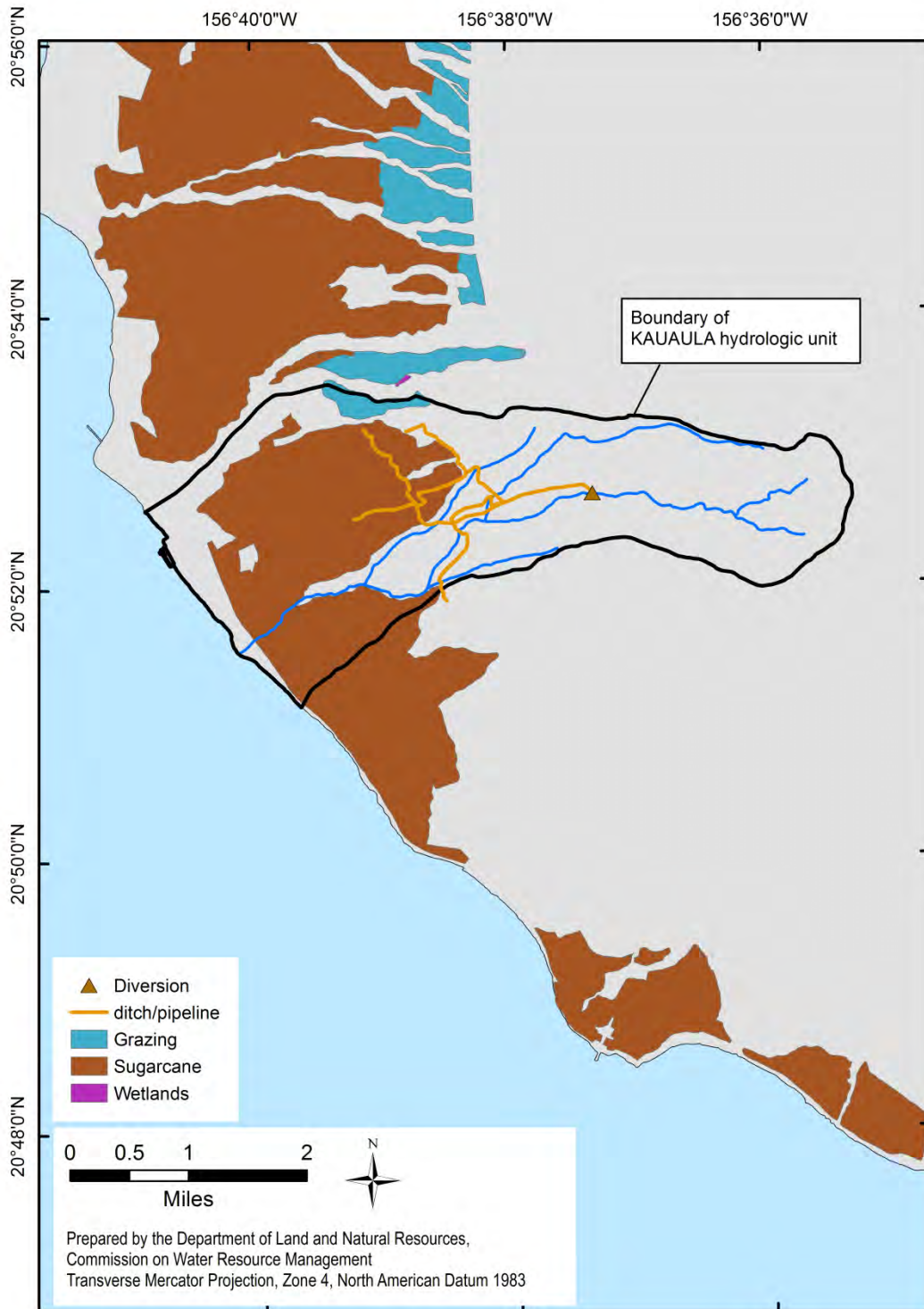
Figure 13-5. Designated agricultural land use for the Kauaula hydrologic unit based on the Agricultural Land Use Map (ALUM). (Source: State of Hawaii, Office of Planning, 2015h)
