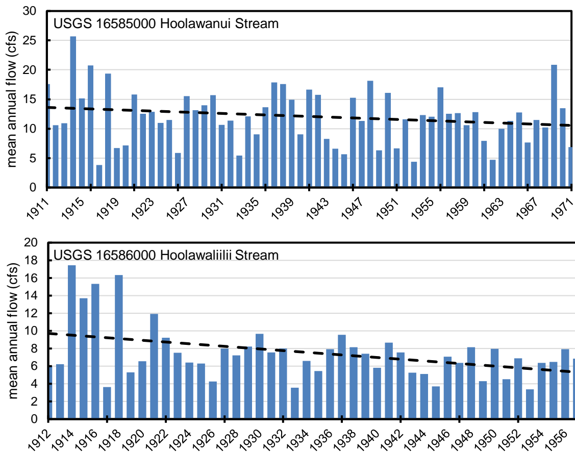
Figure 3-3. Mean annual flow in Hoolawanui Stream at USGS station 16585000 from 1911 to 1971 (top) and in Hoolawaliilii Stream at USGS station 16586000 from 1912 to 1957 (bottom). (Source: USGS, 2020)
