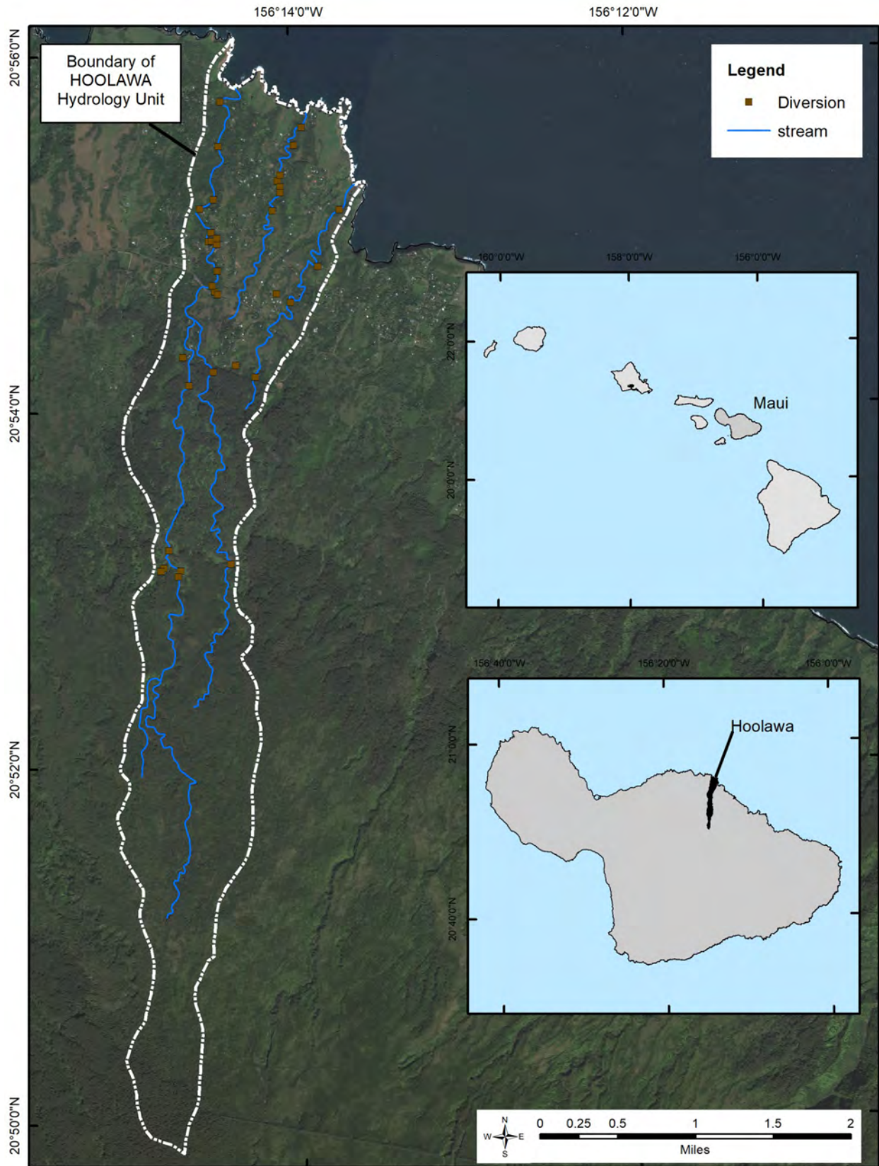
Figure 1-3. Quickbird World View 2 satellite imagery of the Hoolawa hydrologic unit and streams in East Maui, Hawaii.
