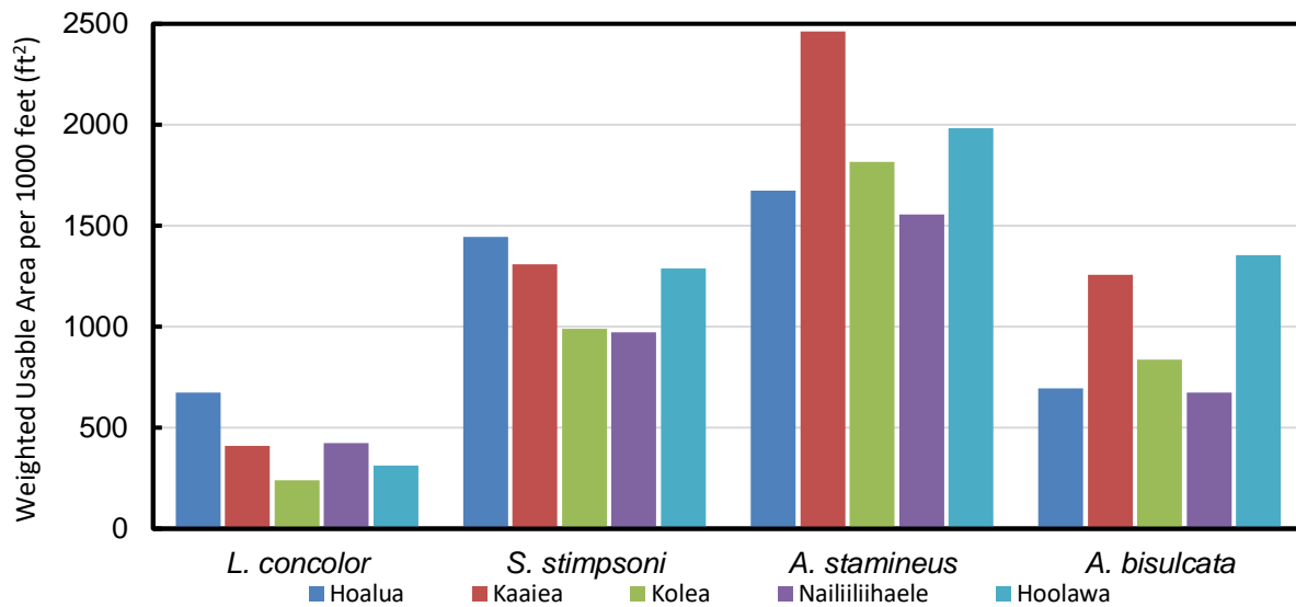
Figure 4-4. Area (ft 2 ) of weighted usable habitat per 1000 feet of stream by species for five non-petitioned streams in the East Maui license area at the 250-foot elevation.
