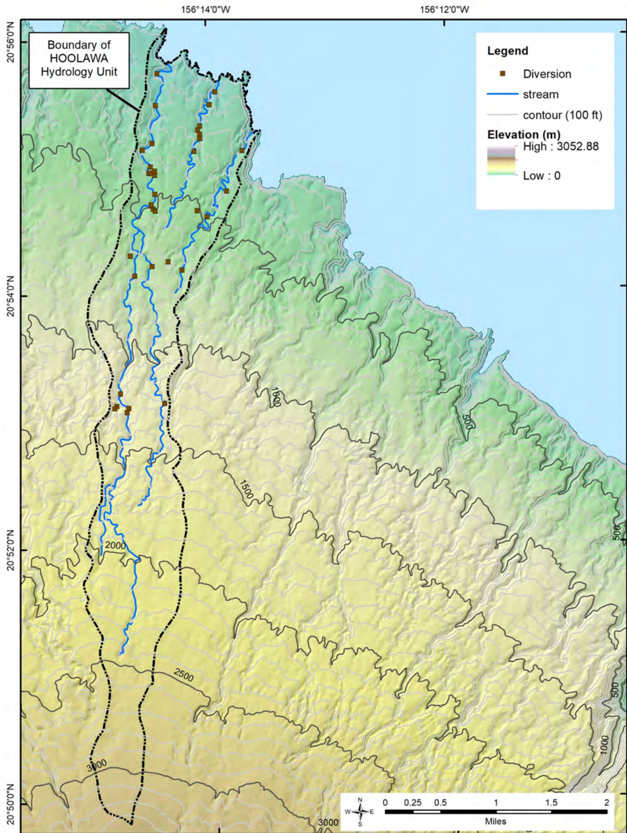
Figure 1-4. Elevation range of the Hoolawa hydrologic unit, Maui. (U.S. Geological Survey, 2001)
