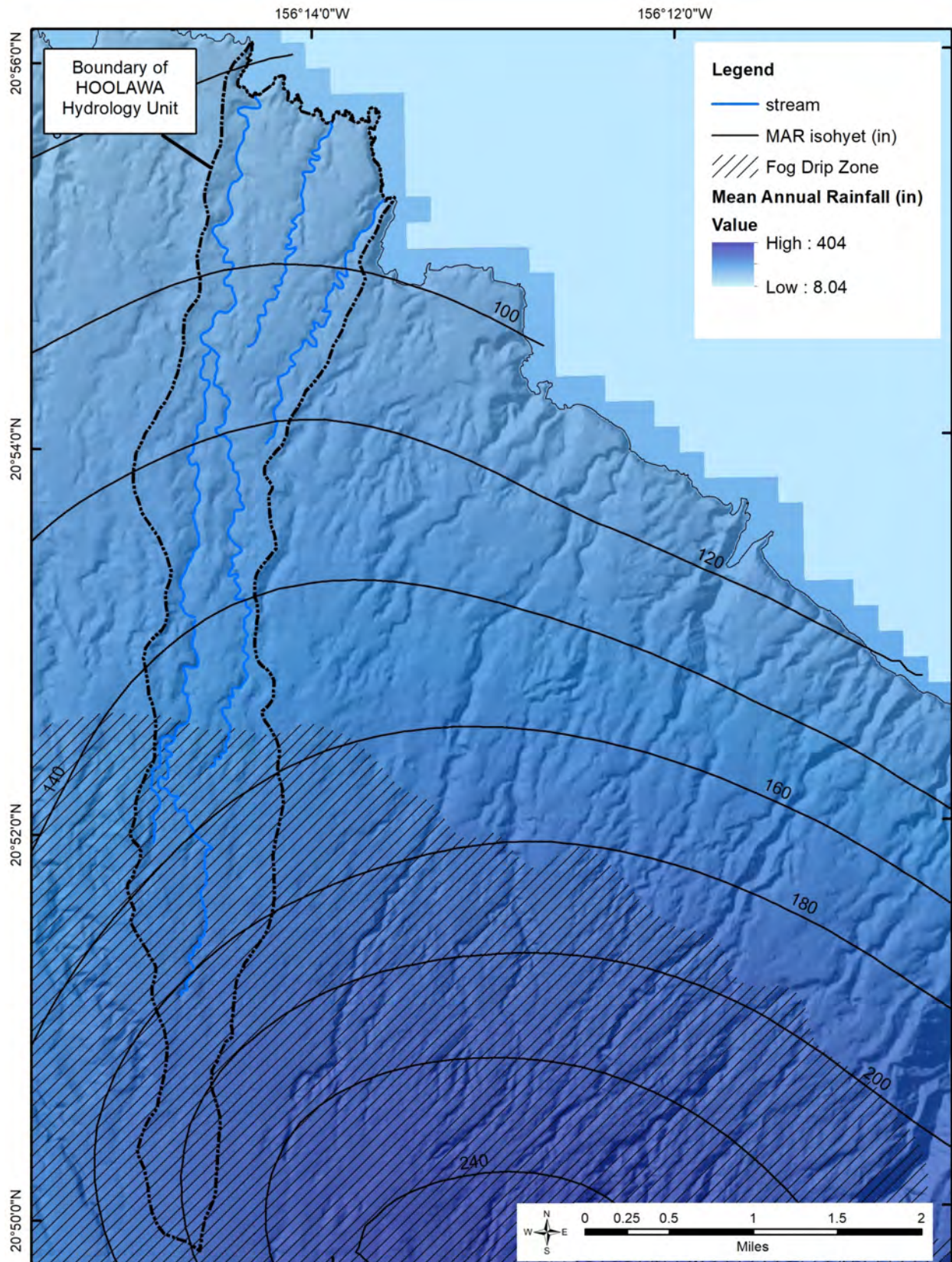
Figure 2-4. Mean annual rainfall and generalized fog drip zone in the Hoolawa hydrologic unit, Maui. (Source: Giambelluca et al., 2013)
