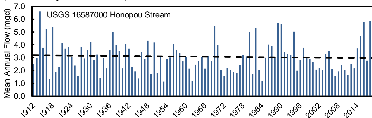
Figure 3-5. Mean annual flow (million gallons per day, mgd) at USGS station 16587000 on Honopou Stream, Maui. Line represents linear regression trend over the period of record. (Source: USGS, 2020)
