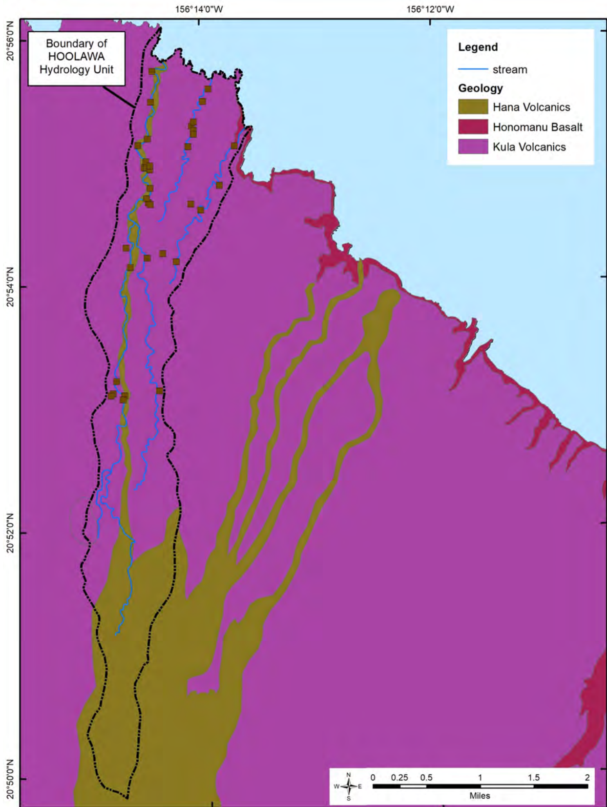
Figure 2-1. Generalized geology of the Hoolawa hydrologic unit, Maui. (Source: Sherrod et al., 2007)
