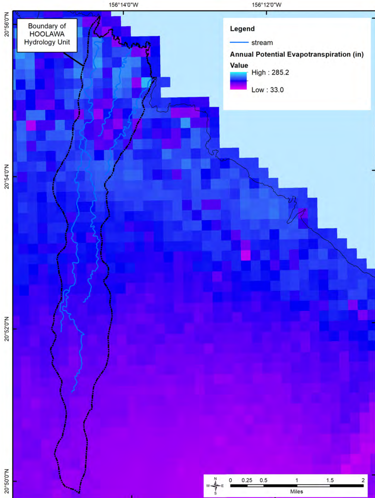
Figure 2-6. Mean annual potential evapotranspiration (Penman-Monteith method) of the Hoolawa hydrologic unit, Maui. (Source: Giambelluca et al., 2014)
