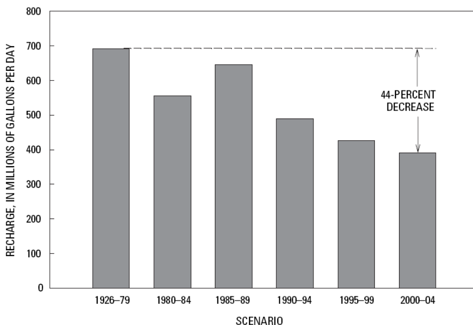
Figure 14-3. Estimated recharge for six historical periods between 1926 and 2004, central and west Maui, Hawaii. (Source: Engott and Vana, 2007)
