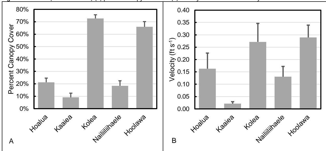
Figure 4-3. Mean ( \pm standard error) (A) percent canopy cover and (B) velocity measured in the surveyed reach
