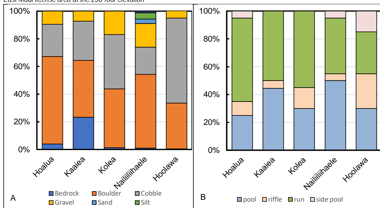
Figure 4-2. Percent of total surveyed area by substrate (A) and habitat classification (B) for five non-petitioned streams in the East Maui license area at the 250-foot elevation
