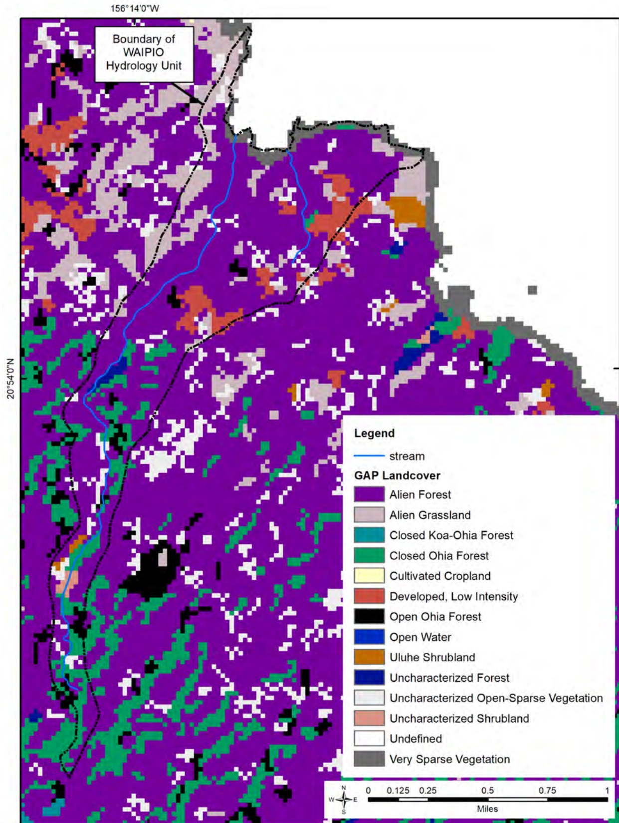
Figure 2-9. Hawaii GAP land cover classes of the Waipio hydrologic unit, Maui (Source: USGS, 2001).
