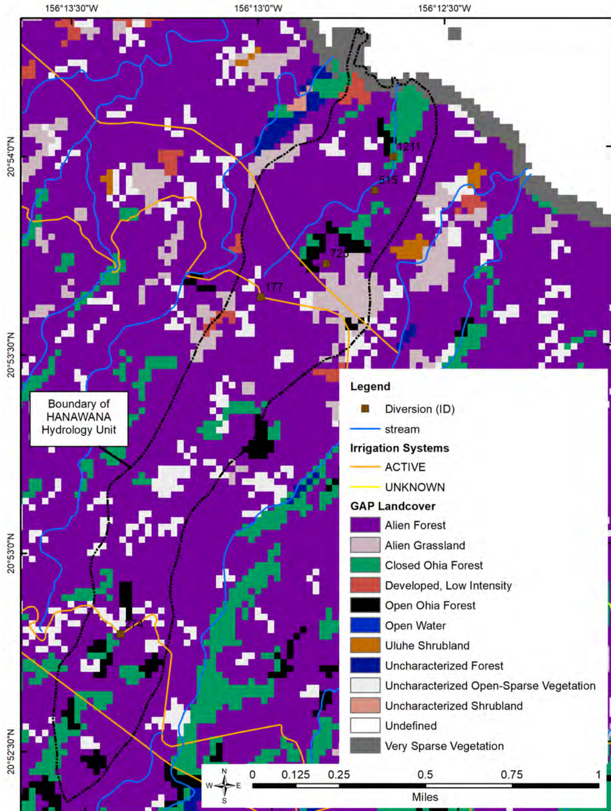
Figure 2-9. Hawaii GAP land cover classes of the Hanawana hydrologic unit, Maui (Source: USGS, 2001).
