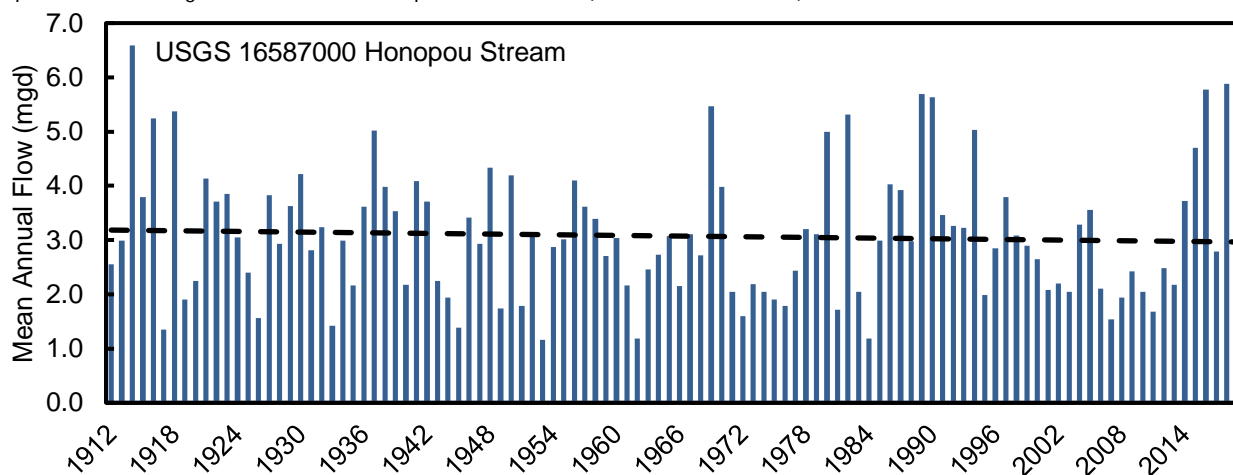
Figure 3-4. Mean annual flow (million gallons per day, mgd) at USGS station 16587000 on Honopou Stream, Maui. Line represents linear regression trend over the period of record. (Source: USGS, 2020)
