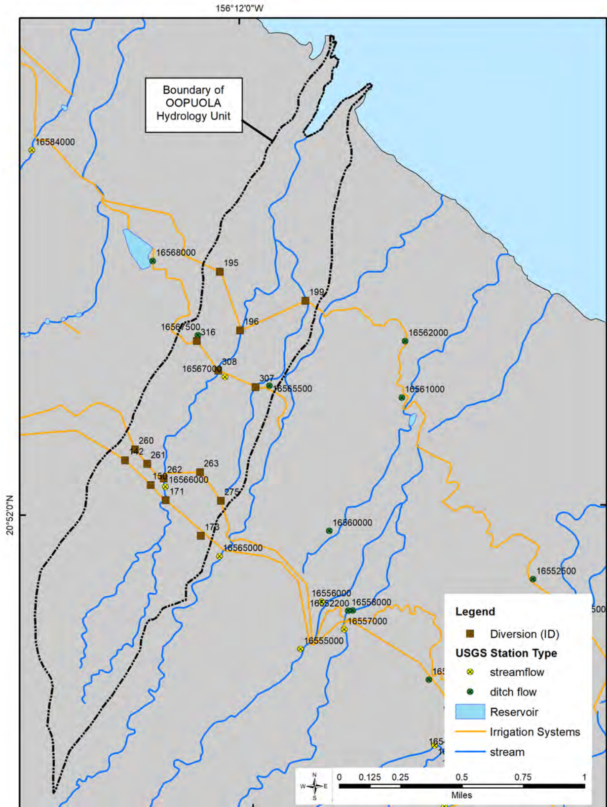
Figure 3-5. Ditches, diversions and USGS gaging stations of streams and ditches in the Oopuola hydrologic unit, Maui. (Source: USGS, 2020).
