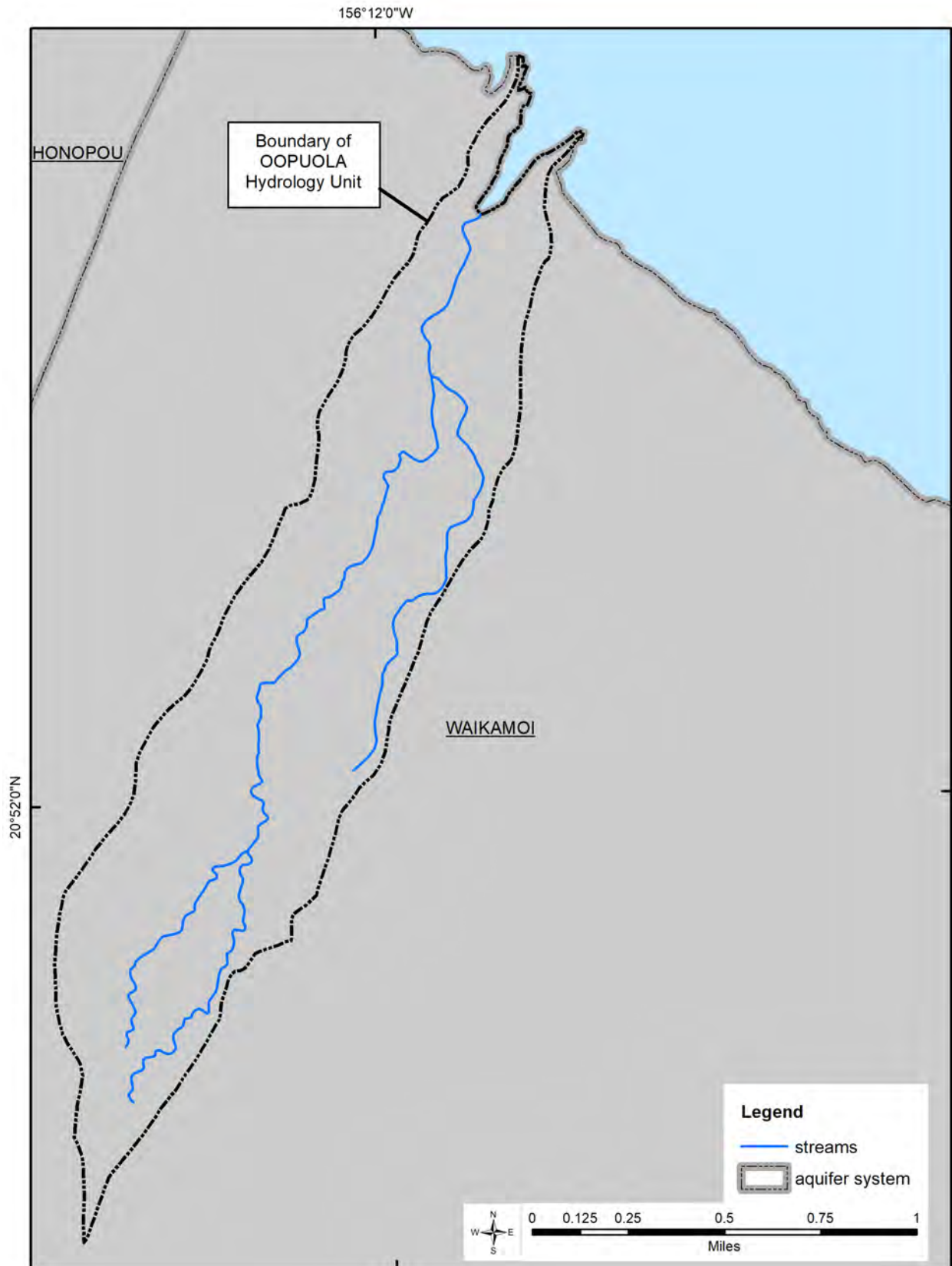
Figure 3-2. The Opuola hydrologic unit in relation to the Waikamoi Aquifer System, Maui. (Source: State of Hawaii, Commission on Water Resource Management, 2020c).
