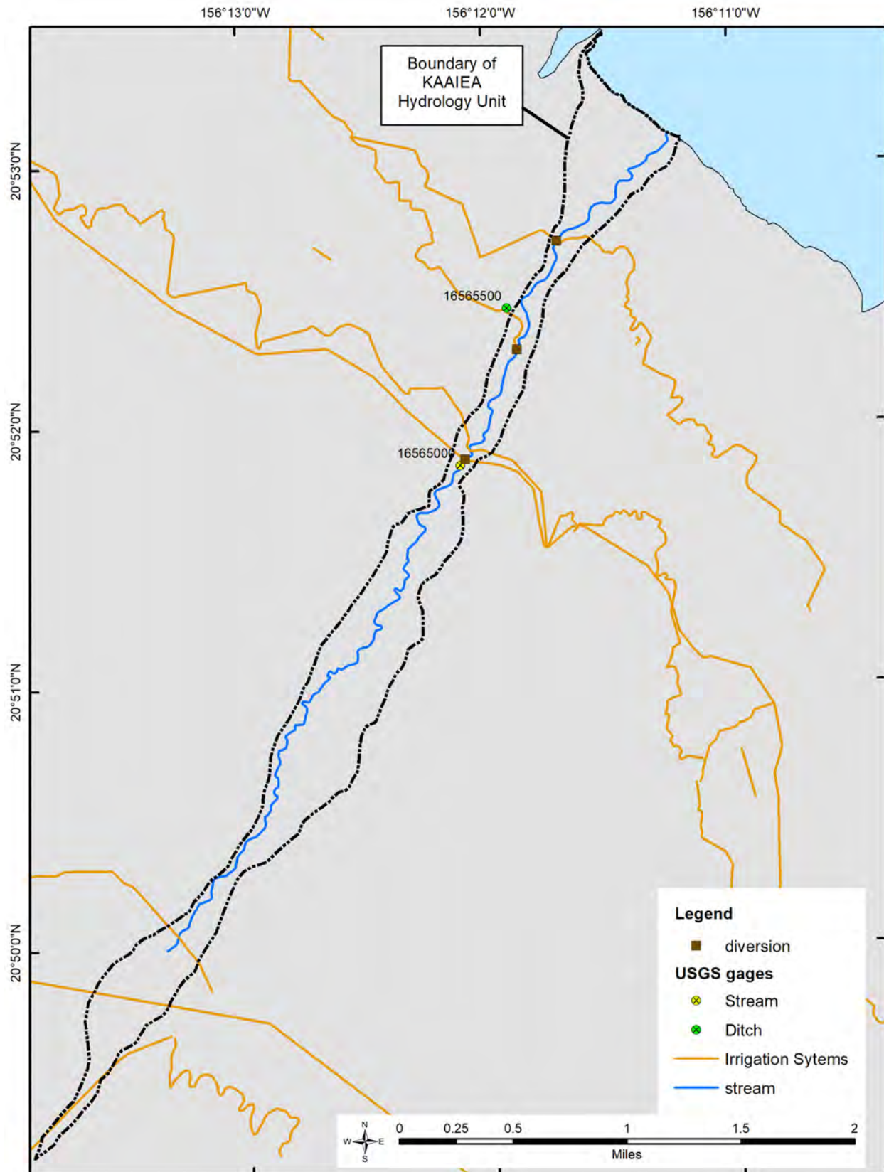
Figure 3-5. Ditches, diversions and USGS gaging stations of streams and ditches in the Kaaiea hydrologic unit, Maui. (Source: USGS, 2020).
