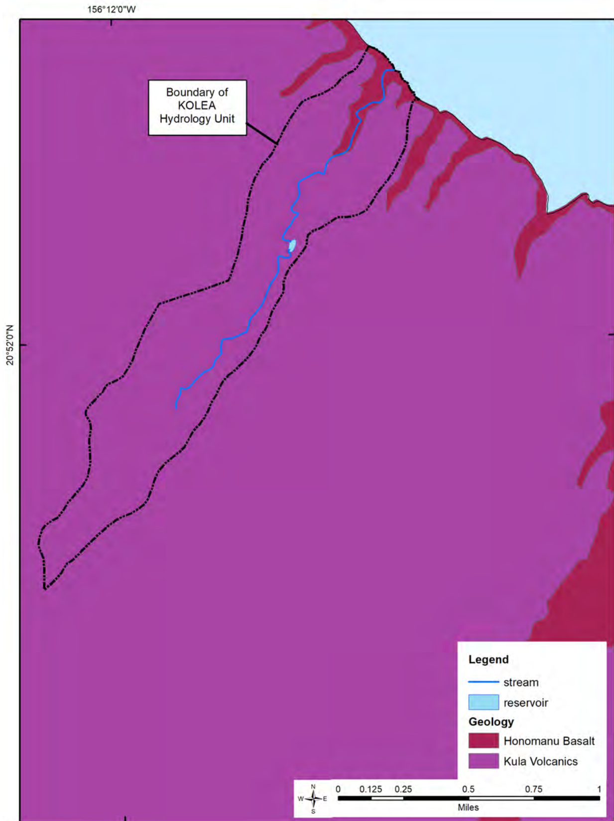
Figure 2-1. Generalized geology of the Kolea hydrologic unit, Maui. (Source: Sherrod et al., 2007)
