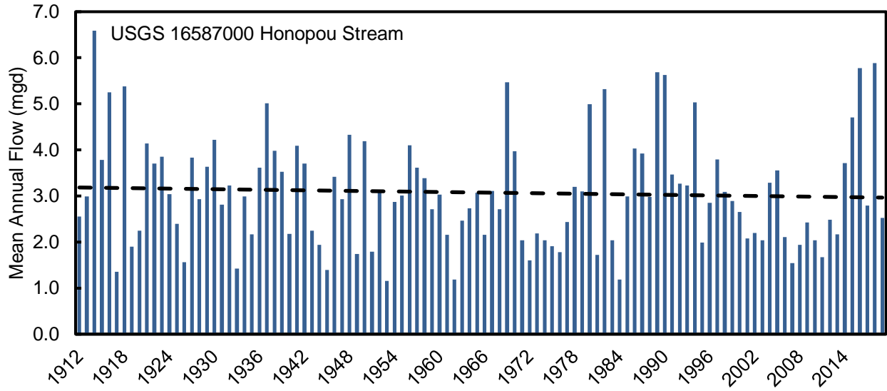
Figure 3-6. Mean annual flow (million gallons per day, mgd) at USGS station 16587000 on Honopou Stream, Maui. Line represents linear regression trend over the period of record. (Source: USGS, 2020)
