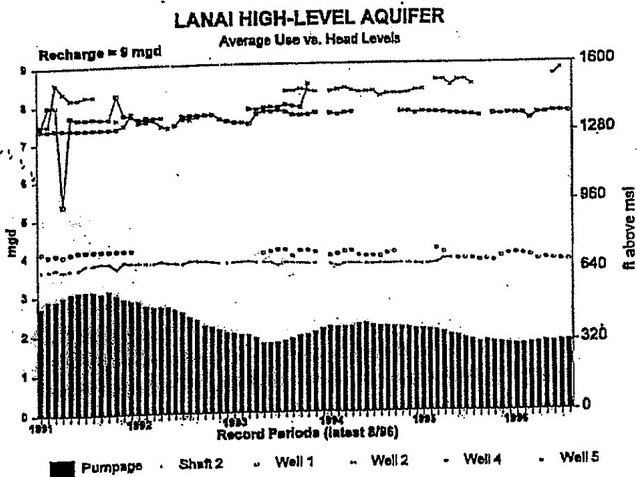
Figure 3. Water levels from 1991 to 1996 (CWRM 18 Oct 96).
