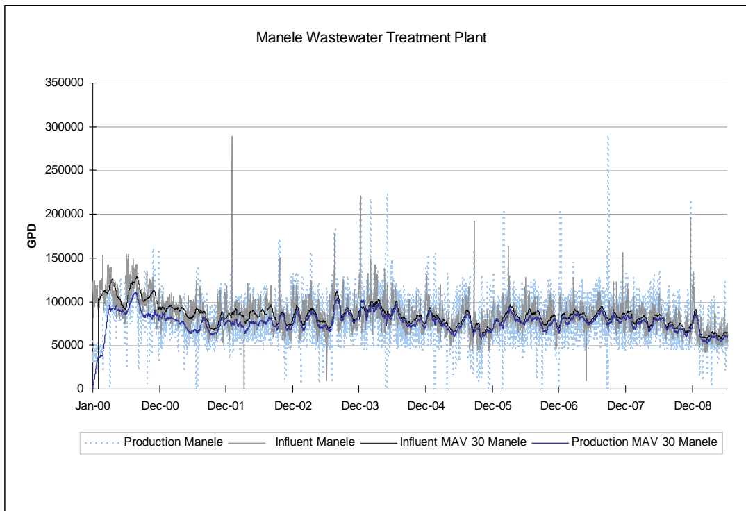
FIGURE 4-27. Manele Wastewater Treatment Plant Flows
