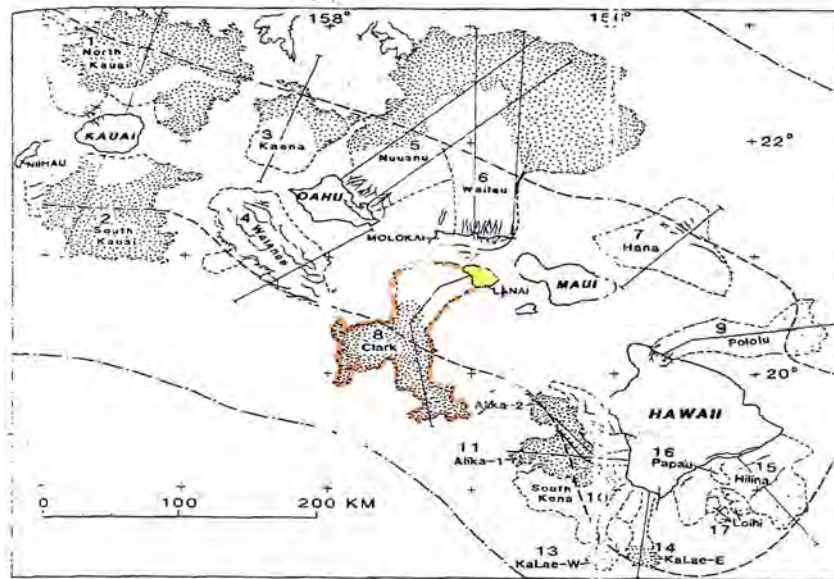
Fig. 2. Map of southeastern Hawaiian Ridge showing major slides bounded by dashed lines identified by number in text and Table 1; compare with Figure 1. Dotted area, hummocky ground (widely scattered where subdued); hachured lines, scarps; thin, downslope-directed lines, submarine canyons and their subaerial counterparts; heavy dashed line, axis of the Hawaiian Deep; dash-dotted line, crest of the Hawaiian Arch.
