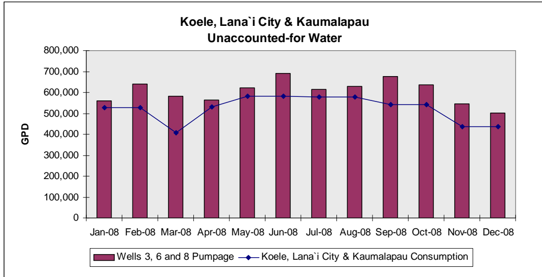
FIGURE 4-19. Unaccounted-for Water in PWS 237 - Koele, Lana'i City & Kaunalapau Regions
