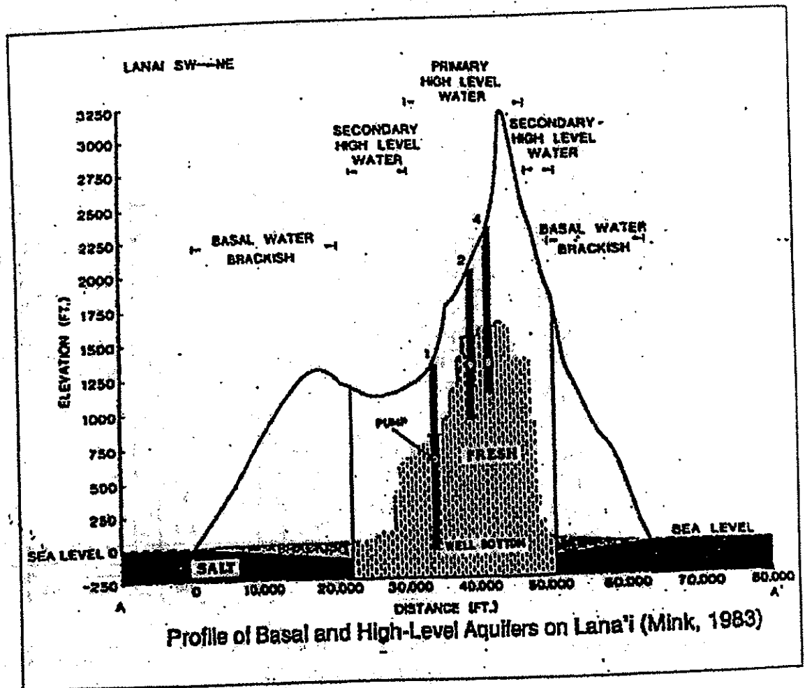
Figure 2. Idealized cross-section of groundwater on Lana'i (CWRM, 19 April 1996).
