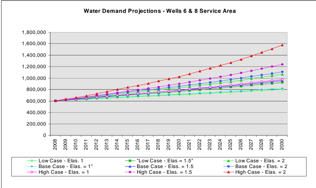
FIGURE 4-40. Wells 6 & 8 Service Area - Projections Using 2008 Pumped Demand
