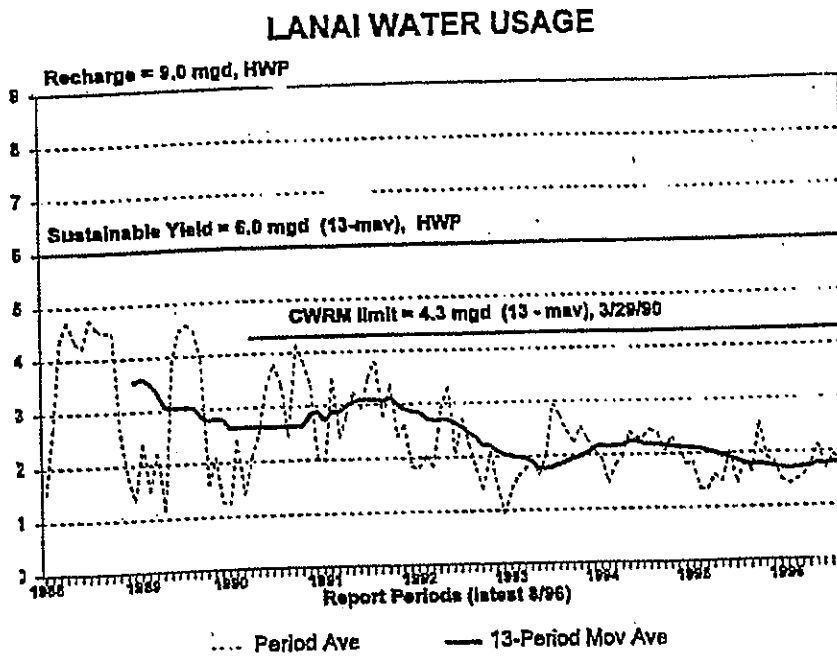
Figure 2. Trend in water usage compared to sustainable yield and CWRM limit (18 Oct 96).
