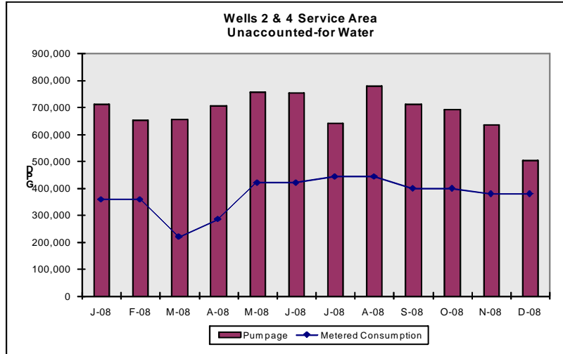
FIGURE 1-8. Pumpage and billing - Palawai grid unaccounted-for water
