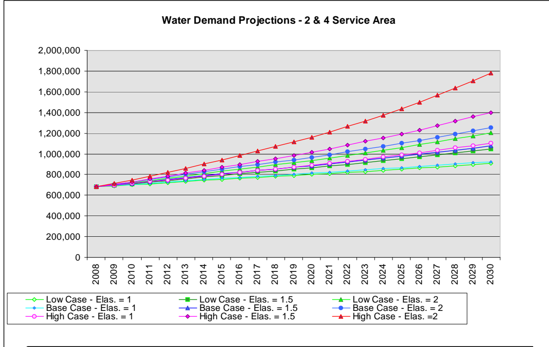
FIGURE 4-42. Wells 2 & 4 Service Area - Projections Using 2008 Pumped Demand
