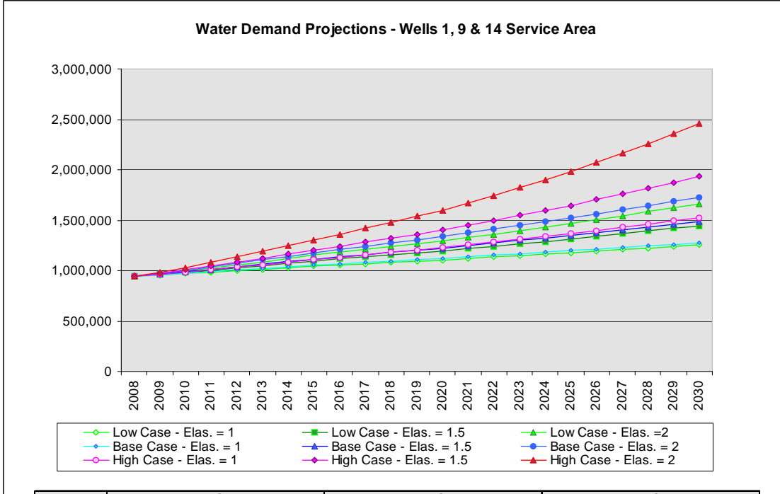
FIGURE 4-44. Wells 1, 9 & 14 Service Area - Projections Using Pumped Demand - Plus 15%
