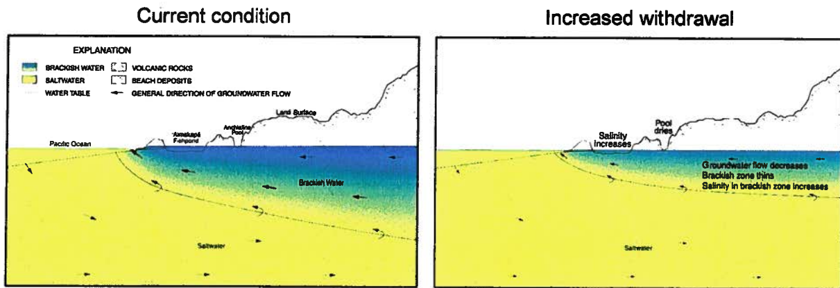
Figure 14. Hydrologic effects of groundwater withdrawals on non-drinking water resources (courtesy of S. Anthony, USGS, 2012). Water levels decline and the saltwater interface rises and moves inland.
