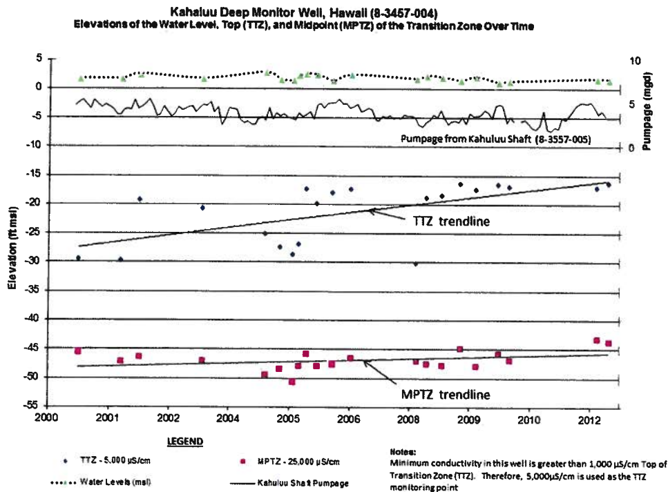
Figure 18. Elevations of the midpoint and top of the transition zone at Kahalu‘u Deep Monitor Well (3457-04) from 2000 to 2012 (from State of Hawaii 2013).
