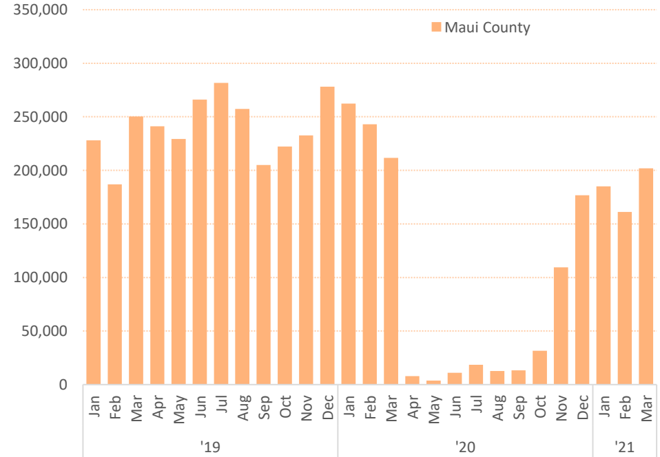
Total airseats
