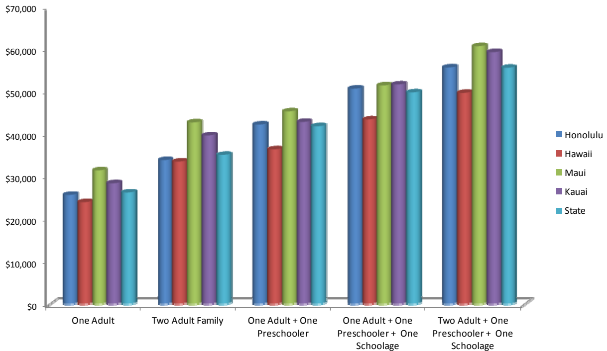
Figure 1. Annual Self-Sufficiency Family Budgets for Selected Family Types, 2009
