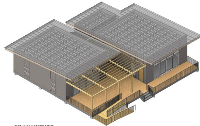
② OVERALL VIEW RAILING OPTION
