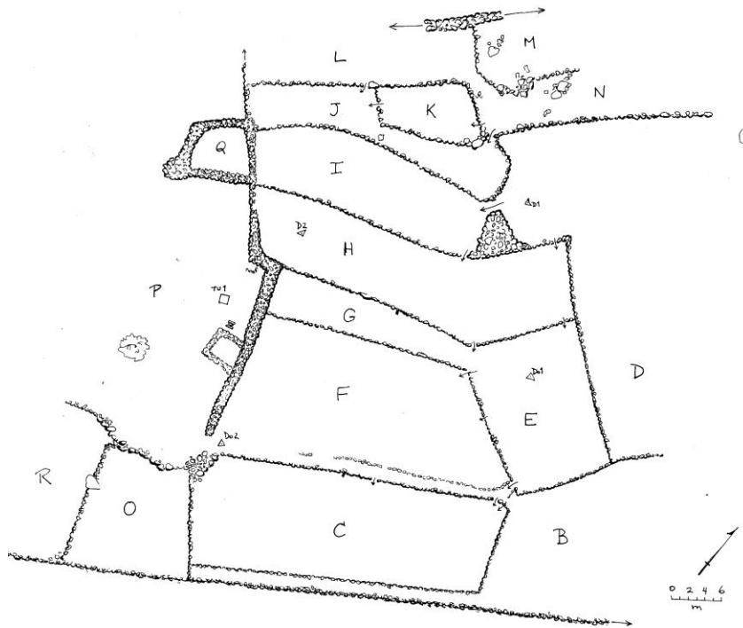
Figure 17. 2005 UH West O‘ahu Field Archaeology class plane table map of a portion of the irrigated kalo terraces in Site 5751. The lower wall is the retaining/boundary wall along the dirt access road into the Cultural Learning Center.
