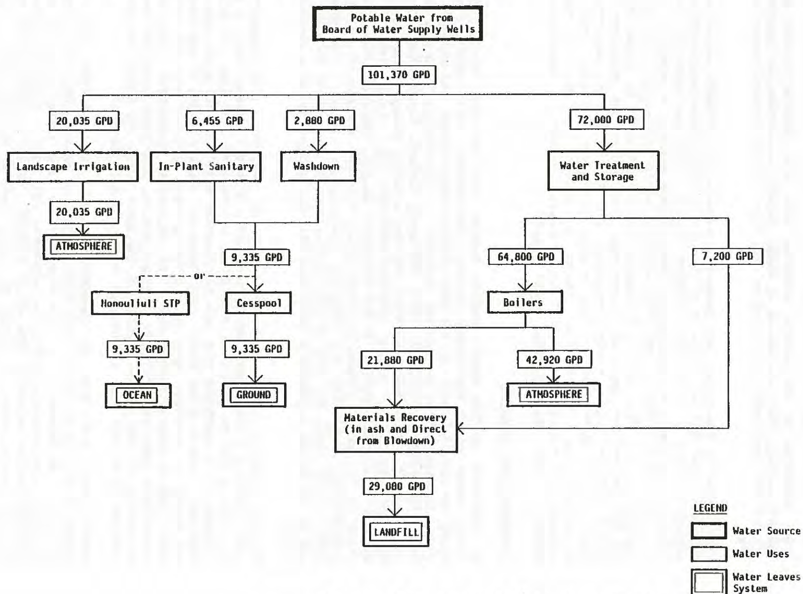
Figure IV-3. Projected Water Balance for the 1,800-TPD HPOWER Facility Proposed By UOP.
