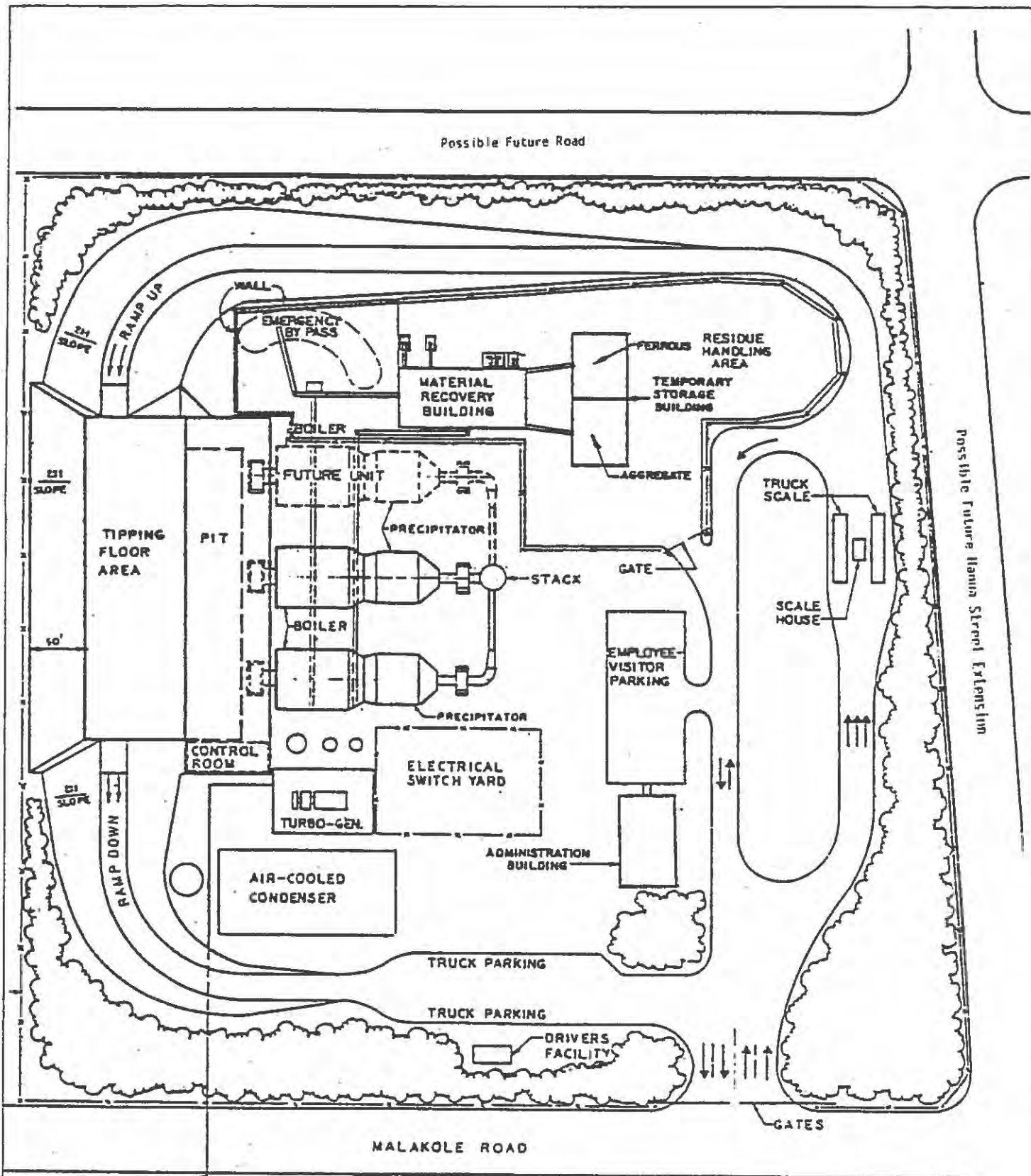
Figure 11-2. Site Layout of the Resource Recovery Facility Proposed by UOP.
