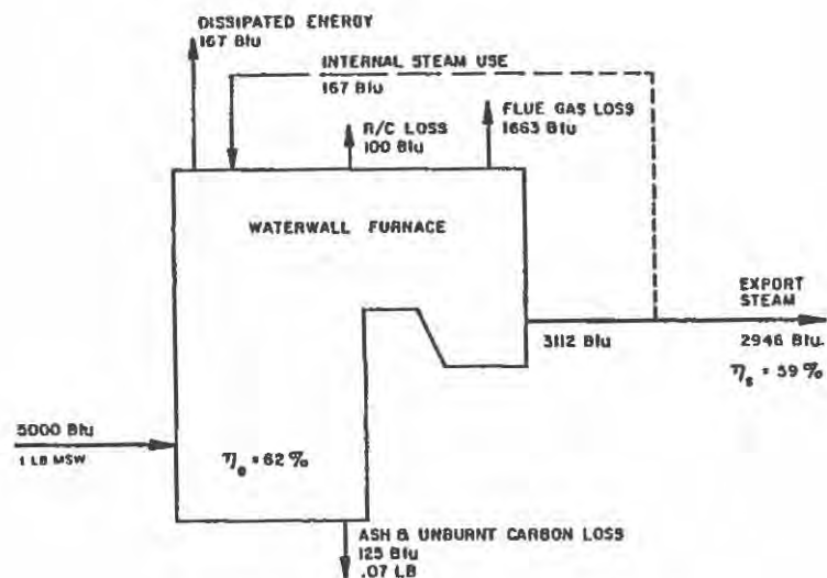
Figure 2. Waterwall Furnace Energy Balance*
