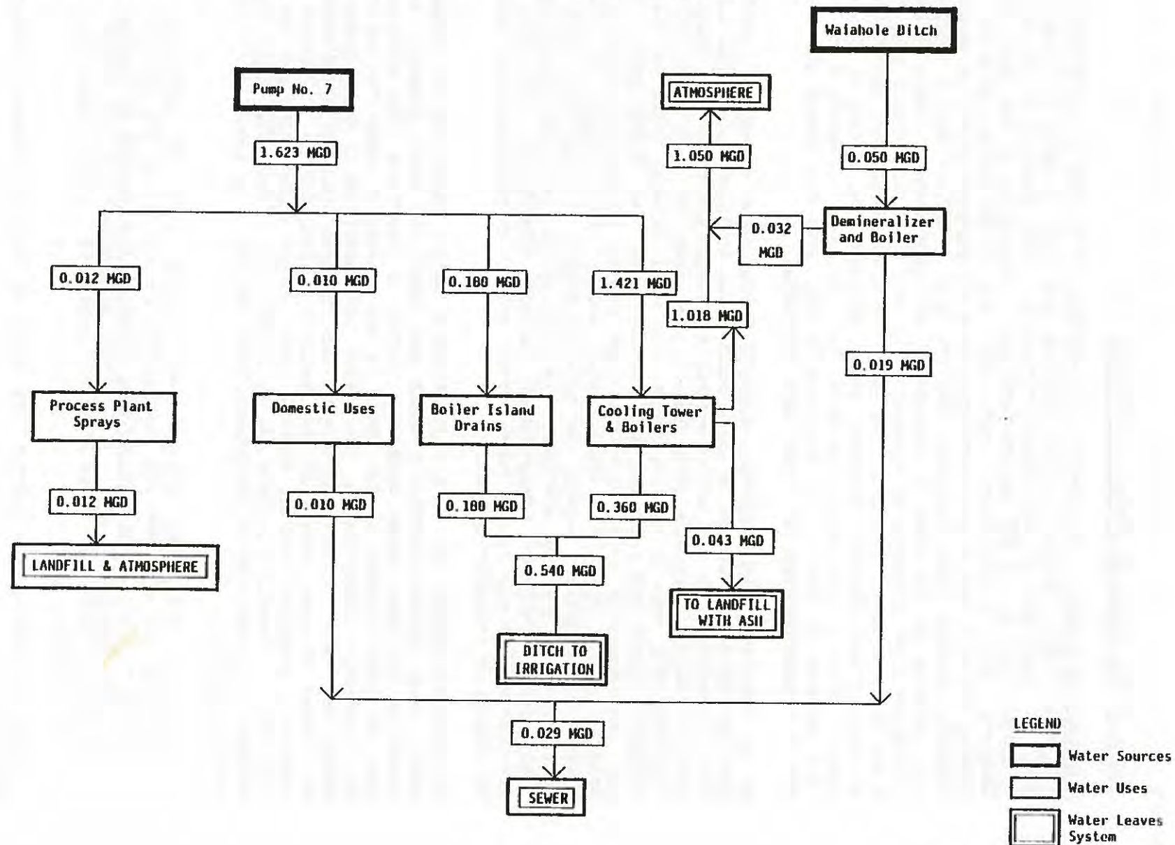
Figure IV-4. Projected Water Balance for the 1,800-TPD HPOWER Facility Proposed by Amfac/C-E.
