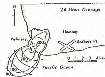
Fig.5 PREDICTED SO 2 - CONCENTRATION ( \mu\text{g}/\text{m}^3 ) AROUND AN OIL REFINERY
