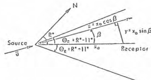
Fig. 2: Geometry of a 1° Sector Model
