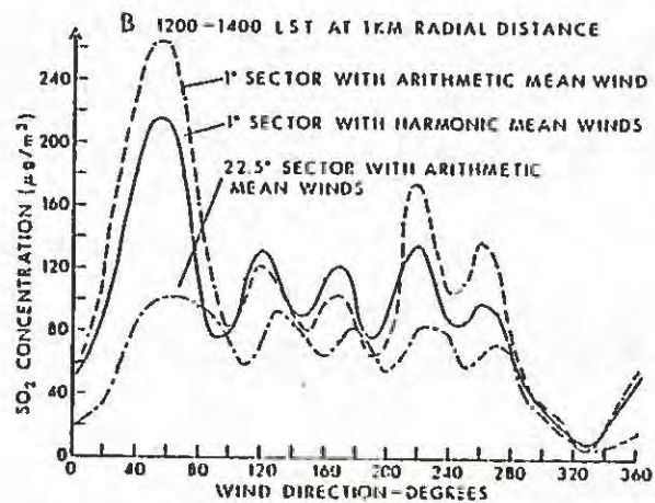
Fig.3A&B SO 2 CONCENTRATIONS AS CALCULATED USING DIFFERENT METHODS
