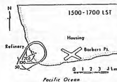
Fig.4 PREDICTED SO 2 - CONCENTRATION ( \mu\text{g}/\text{m}^3 ) AROUND AN OIL REFINERY
