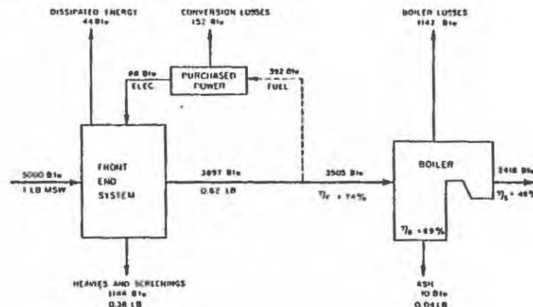
Figure 4. Fluid RDF Energy Balance*
