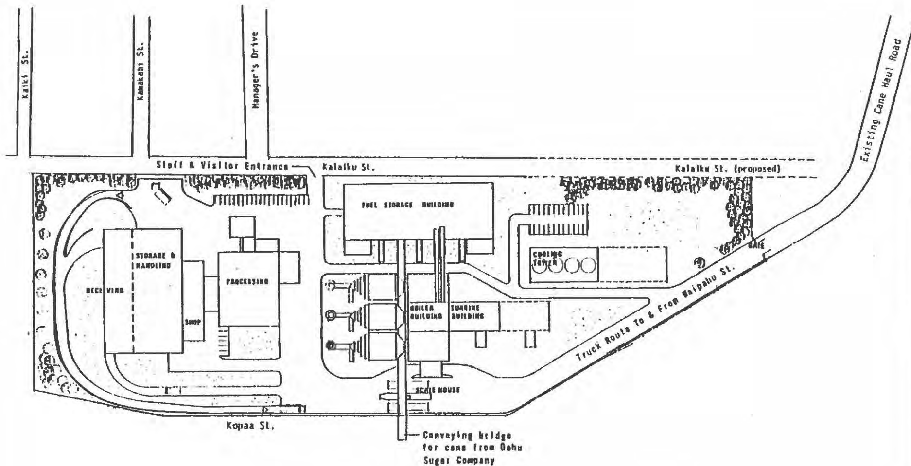
Figure II-5. Site Layout of the Resource Recovery Facility Proposed by Amfac/C-E.
