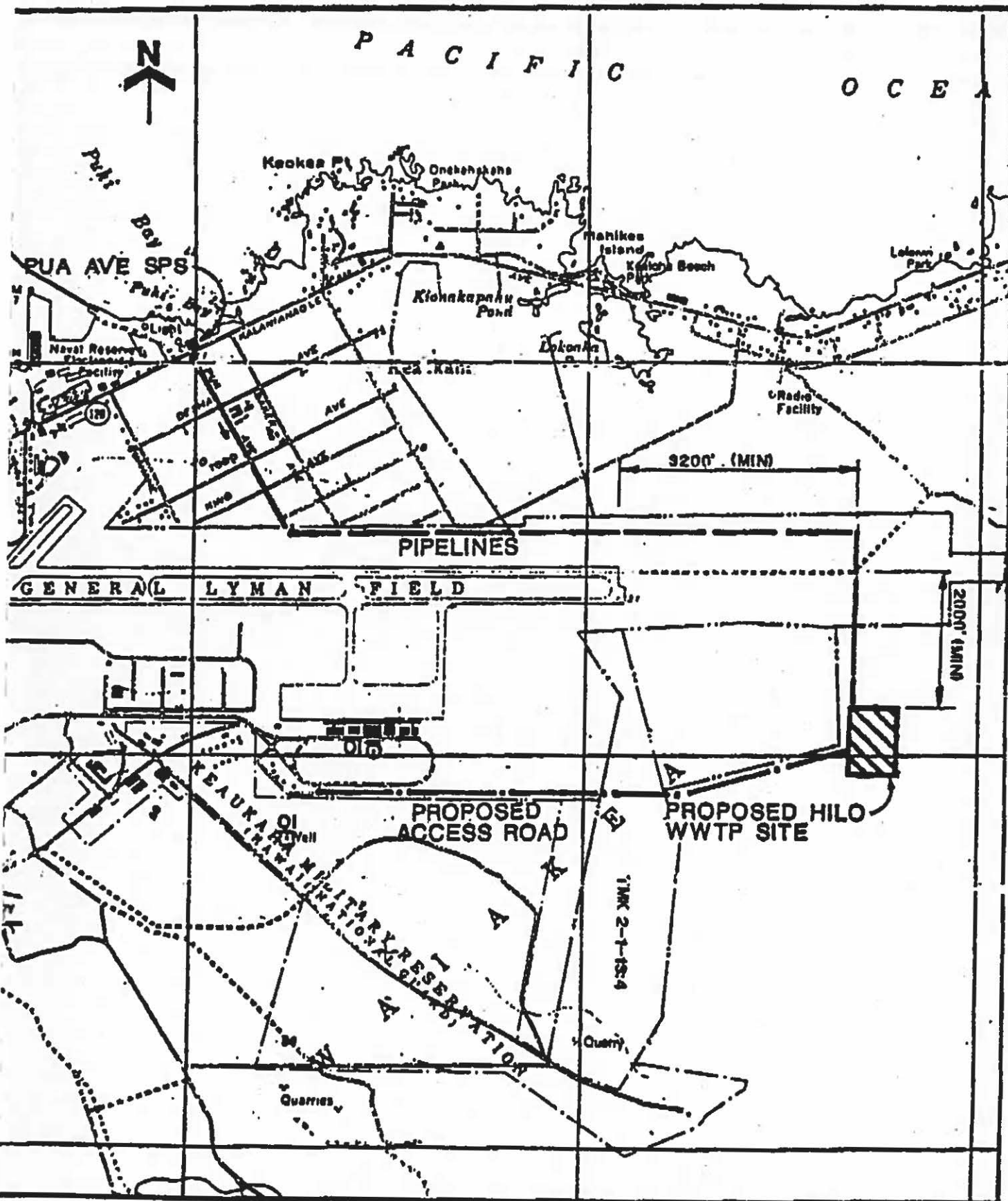
HILO WASTEWATER TREATMENT PLANT SITE SCALE: 1" = 2000'
