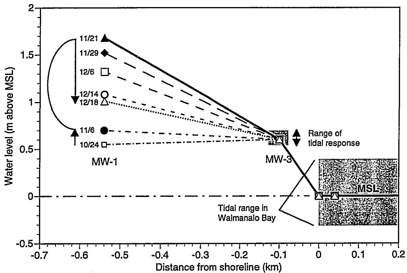
Figure 3. Groundwater heads across the MW-1/3 transect. The MW-1 head increased significantly following the 11/15-16 storm, then declined continuously through 12/18. After 12/18, the water level in MW-1 fluctuated in response to a series of moderate storms. MW-3 was not significantly affected by changes in water input to the watershed, staying within a relatively narrow range coincident with the range defined by the response to tidal forcing measured by MGD, Inc. Groundwater head gradients between MW-1 and MW-3 varied from -0.01% on 10/24 to +0.25% on 11/21. The gradient between MW-3 and the ocean (MSL) remained essentially constant at +0.6%. MW-2 and MW-4 heads responded very similarly to MW-1 and MW-3, respectively, with absolute post-storm heads slightly lower than shown above.
