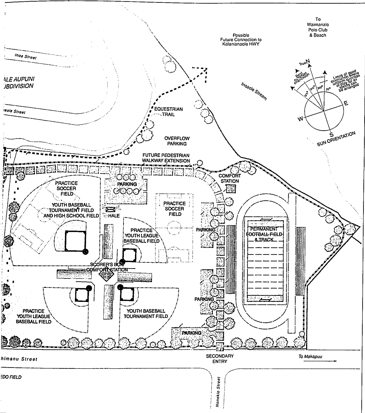
FIGURE 5 MASTER PLAN Waimanalo District Park
