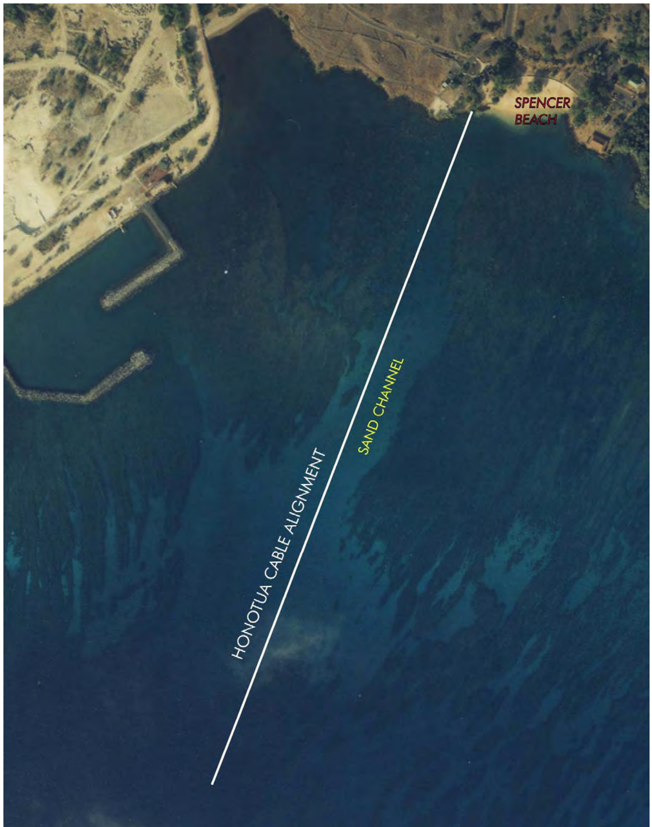
FIGURE 1. Aerial photograph of Spencer Beach and offshore area showing approximately alignment of Tahiti-Hawaii Honotua Cable. Also shown is location of sand channel that extends to the shoreline.
