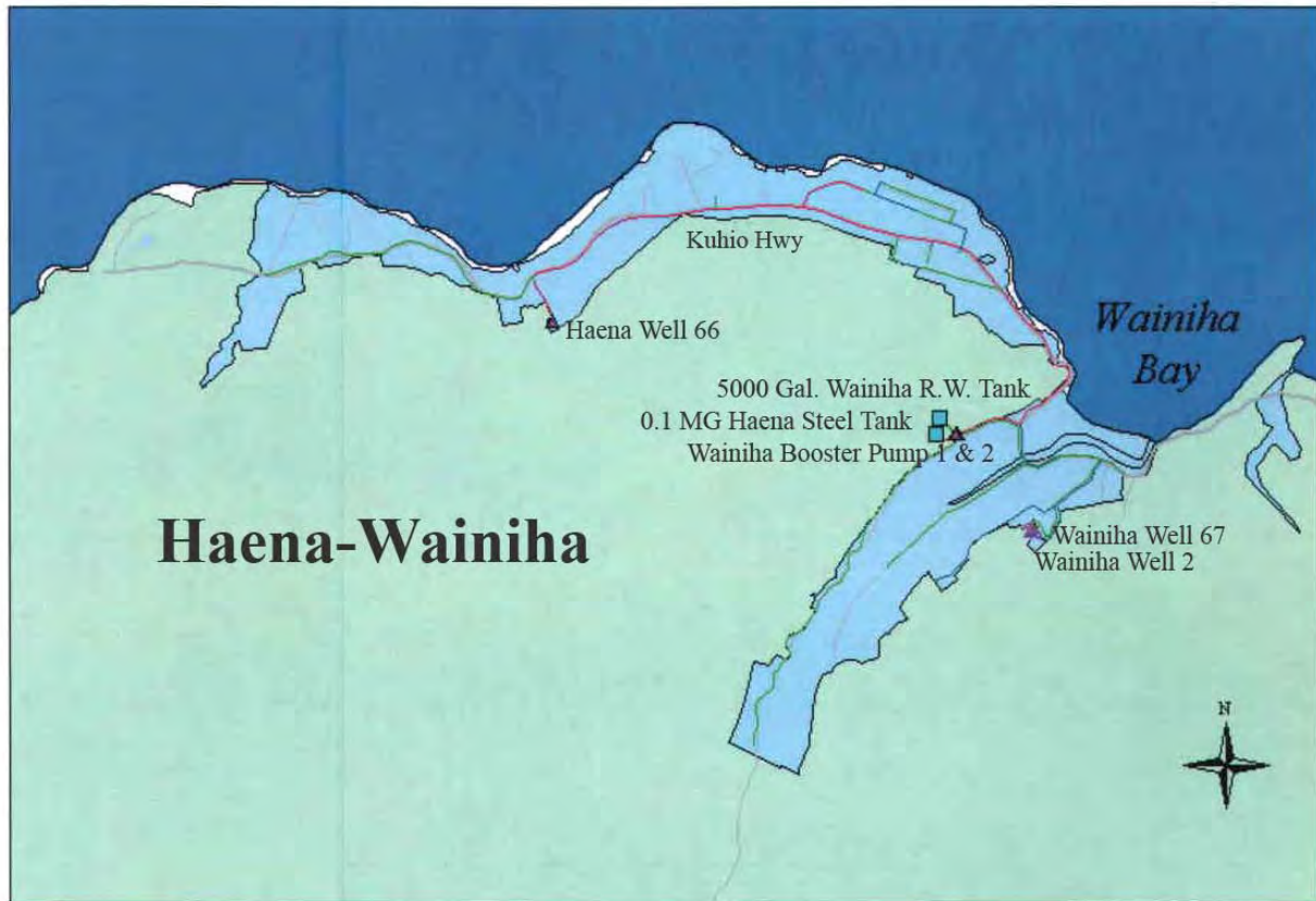
Figure 9 Wainiha-Hā'ena Existing Water System
