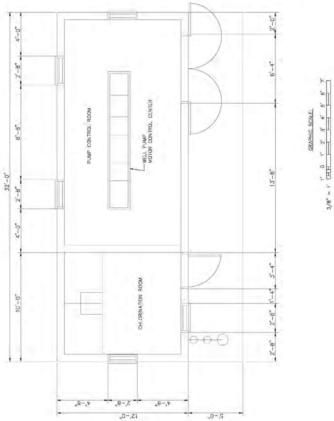
Figure 6 Wainiha Water Well Pump Control Building Plan
