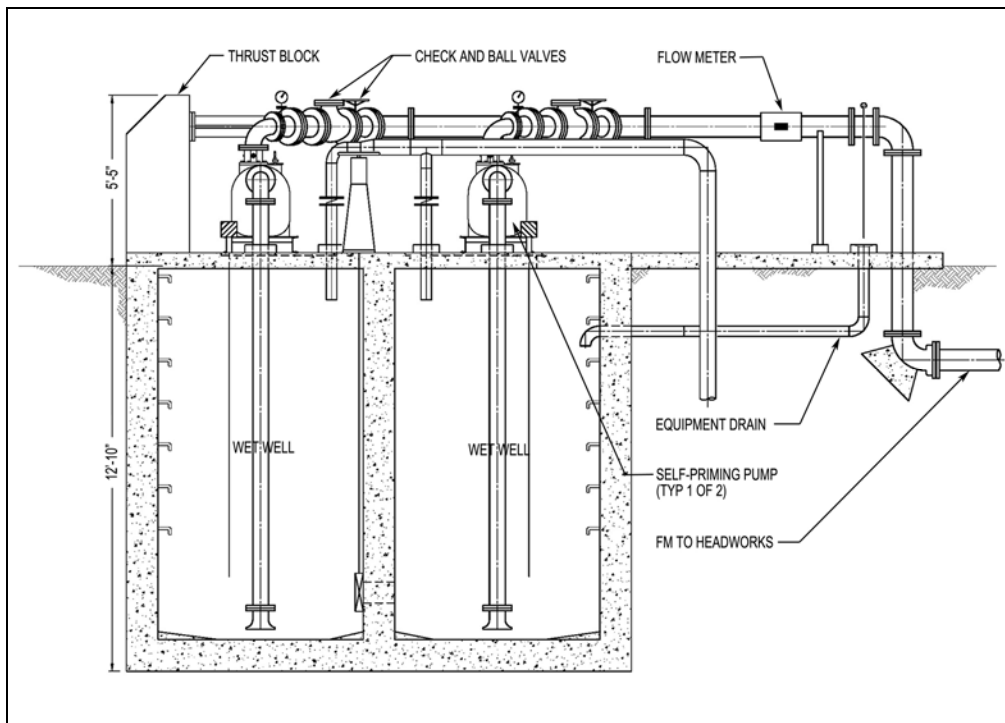
Figure 2-5 New Solids Handling Building Return Lift Station Section
