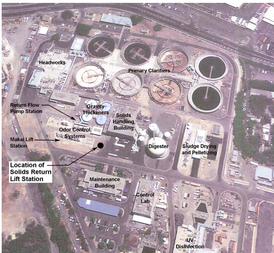
Figure 2-1 Aerial View of Sand Island WWTP
