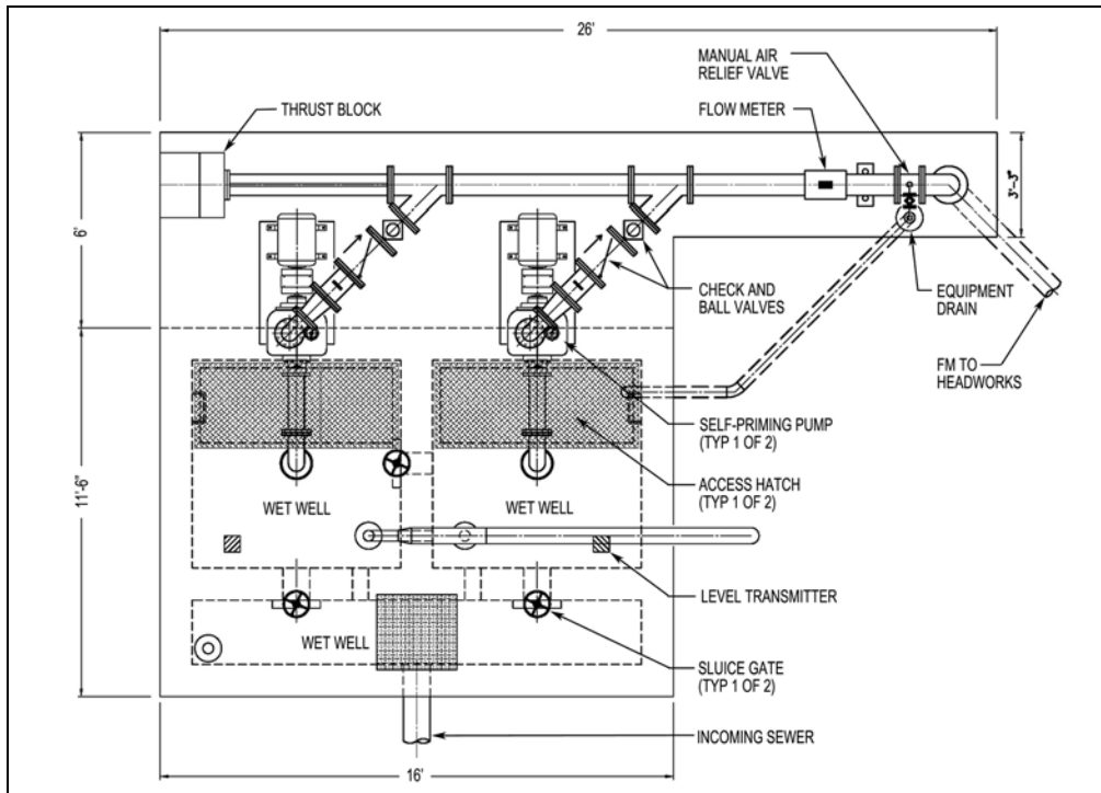
Figure 2-4 New Solids Handling Building Return Lift Station Plan View
