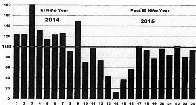
Figure 4a. Average rainfall, % of monthly mean, for a composite of historical El Niño years and the years following El Niño for Majuro. Note that during El Niño there is abundant rainfall, with some very high monthly values. Dryness starts late in the El Niño year, and worsens in the first few months of the year following El Niño. This chart is not a specific forecast, but represent plausible rainfall behavior at Majuro for 2014 and 2015. Drought severity and recovery of rainfall after El Niño varies from island to island.
