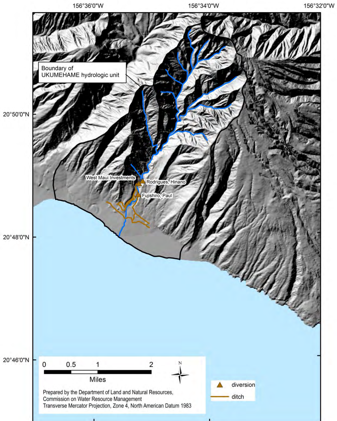
Figure 13-2. All diversions and ditches identified in the Ukumehame hydrologic unit. (Source: State of Hawaii, Office of Planning, 2004d; State of Hawaii, Commission on Water Resource Management, 2015g)
