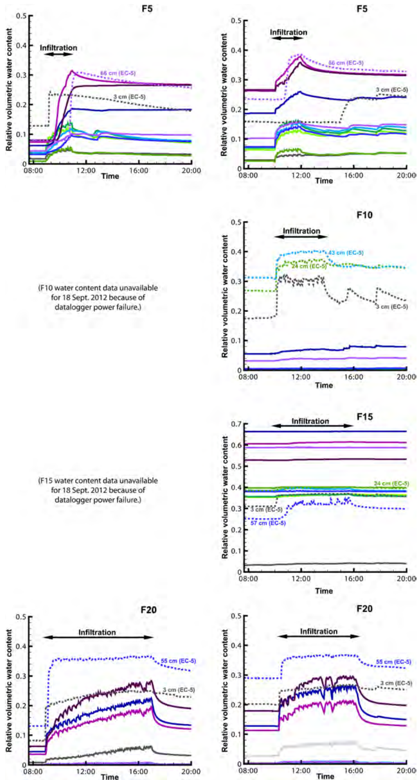
Figure 7. Response to the 18 September 2012 ('dry' application, left column) and 19 September 2012 ('wet' application, right column) artificial infiltration event of water content sensors. Graphs are ordered in increasing magnitude of treatment (5.1 cm at the top to 20.3 cm at the bottom). Response at different depths is indicated by different-coloured lines. Solid lines indicate Sentek EnviroSCAN sensors and dashed lines indicate Decagon EC-5 sensors. Enviroscan water content sensors were installed at 10–100-cm depth, as indicated in the legend. Sites F10, F15, G5, G10, G15, and G20 have sensor depths that are offset from the legend (Table III). Note that the absolute value differences between the probe types is because of factory calibration. The period of infiltration at each plot is marked with a horizontal line.
