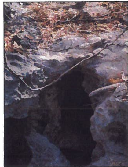
Figure 3.1. Karst topography and sinkholes within the project site.
