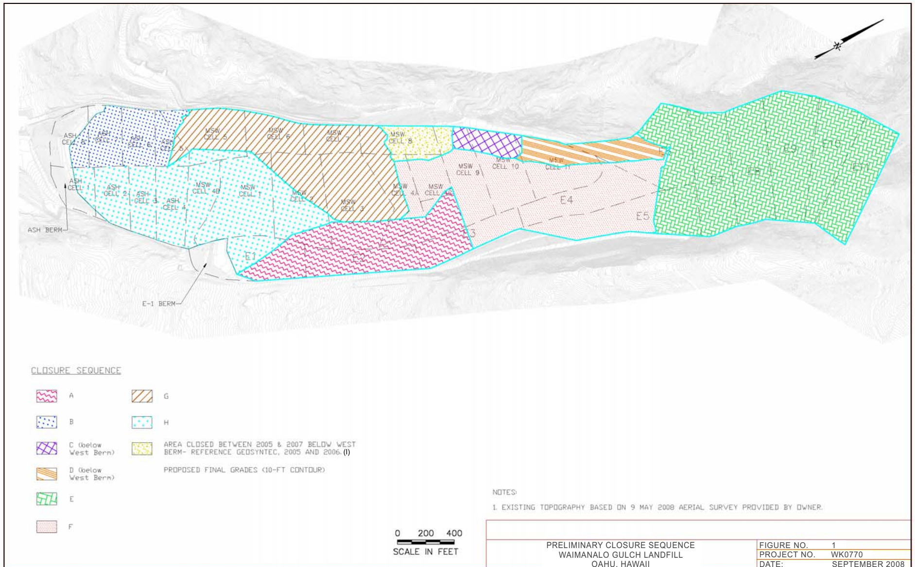
Figure 4-9 Preliminary Closure Sequence Waimanalo Gulch Sanitary Landfill Expansion Department of Environmental Services
