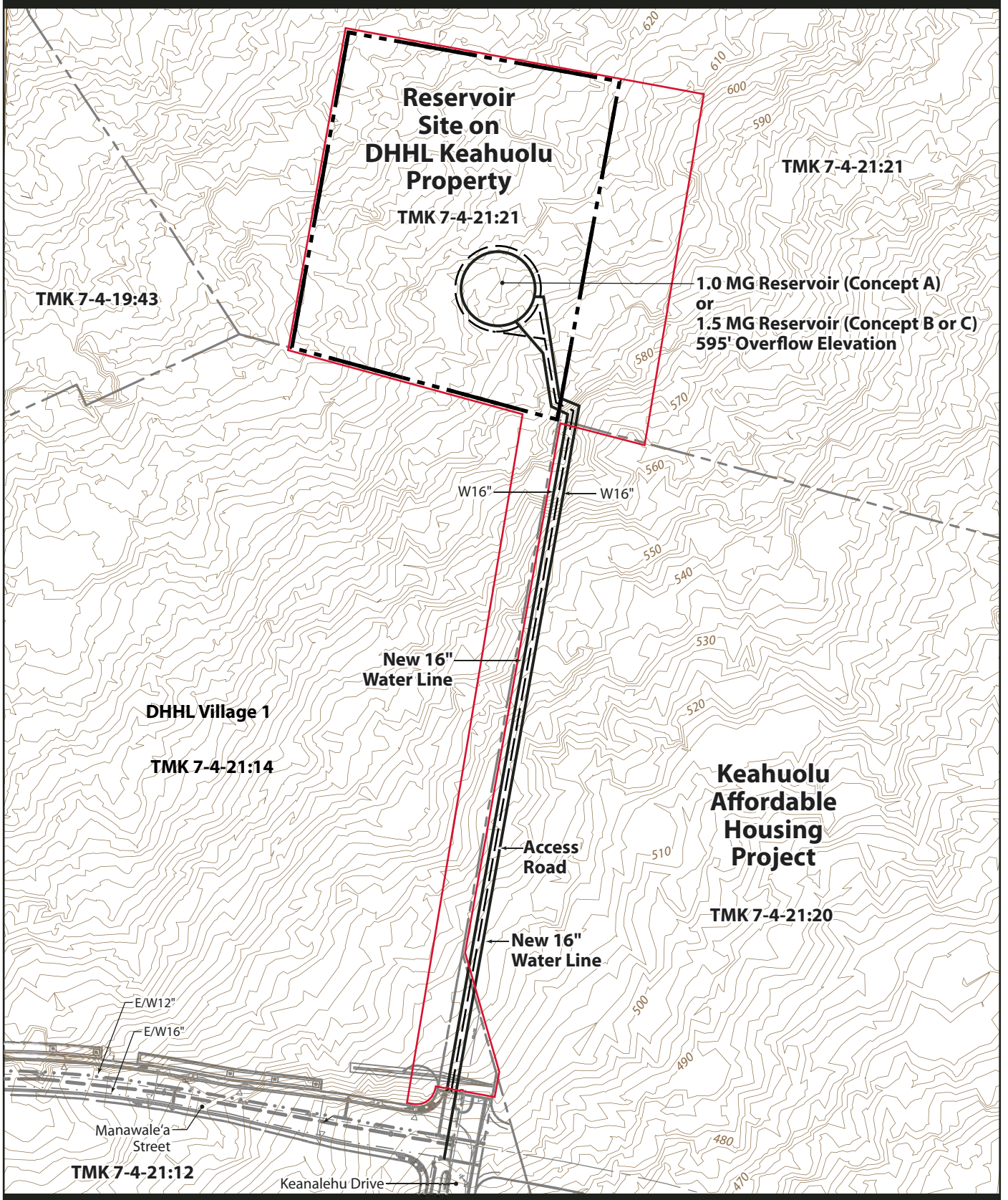
Figure 3-7 RESERVOIR ON DHHL KEAHUOLU PROPERTY
