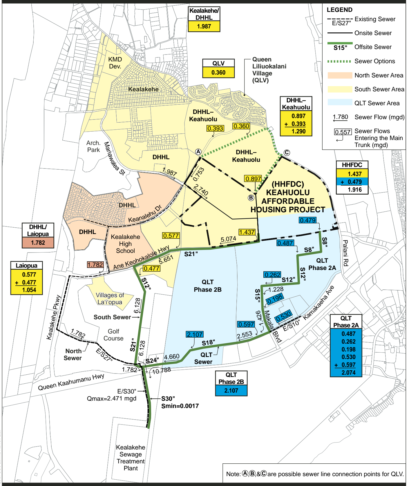
Figure 3-10 OFFSITE SEWER SYSTEM CONCEPT A—LA'IO'OPUA ROUTE
