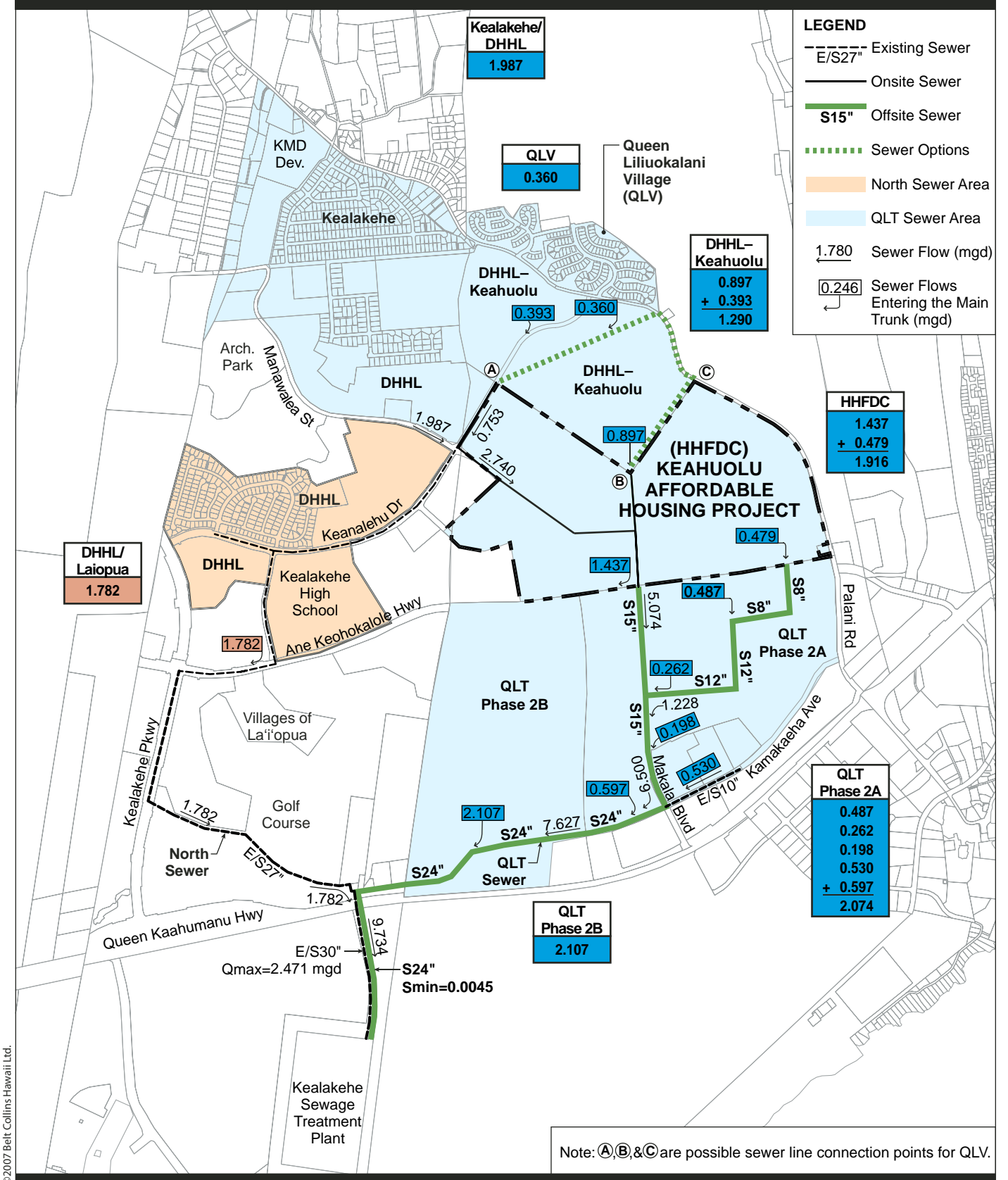
Figure 3-8 OFFSITE SEWER SYSTEM CONCEPT A—QLT ROUTE
