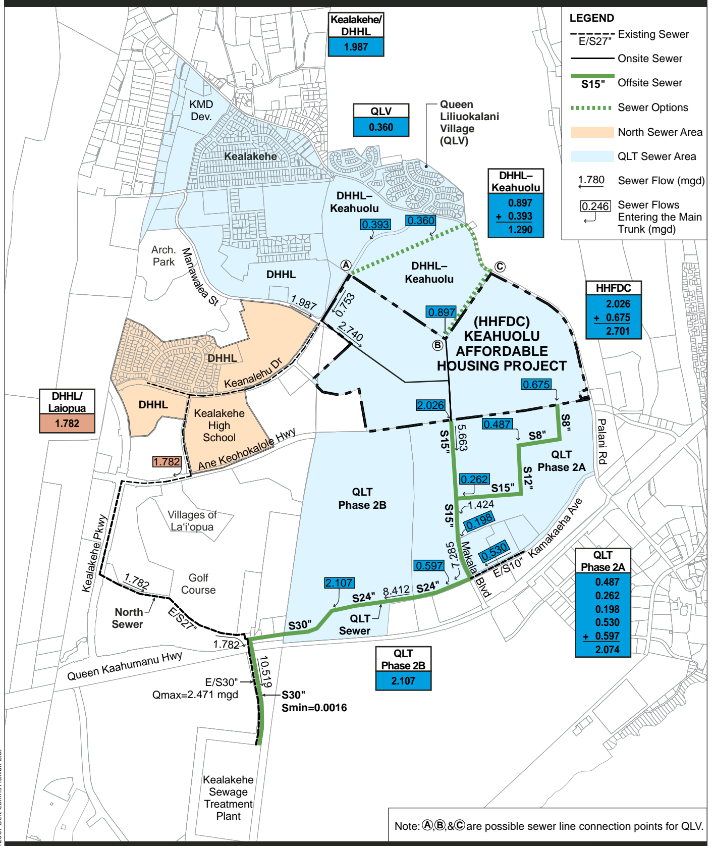
Figure 3-9 OFFSITE SEWER SYSTEM CONCEPTS B & C—QLT ROUTE
