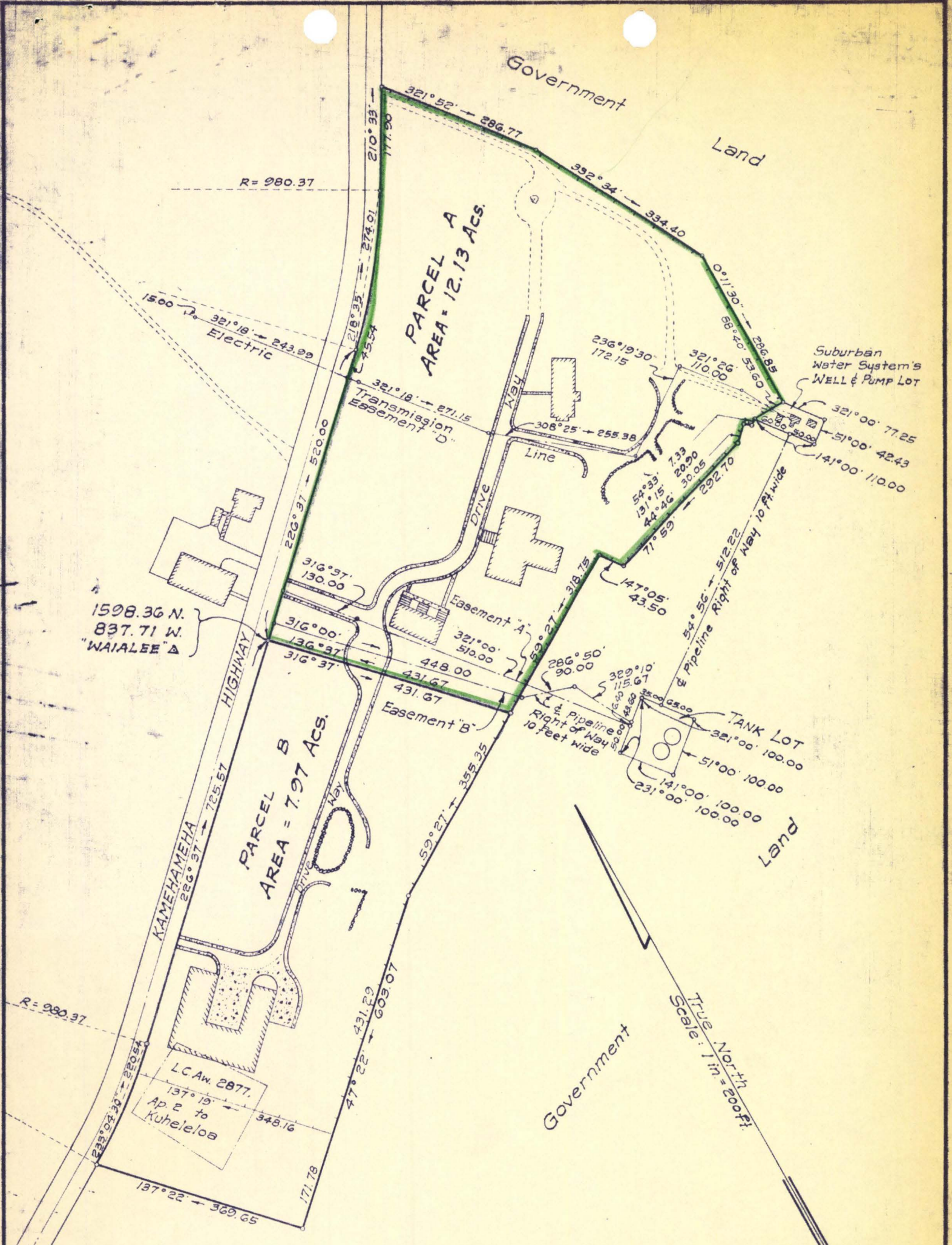
Old Waialeale Boys School PARCELS A and B Waialeale, Koolauloa, Oahu, T.H. Scale: 1 inch = 200 feet
