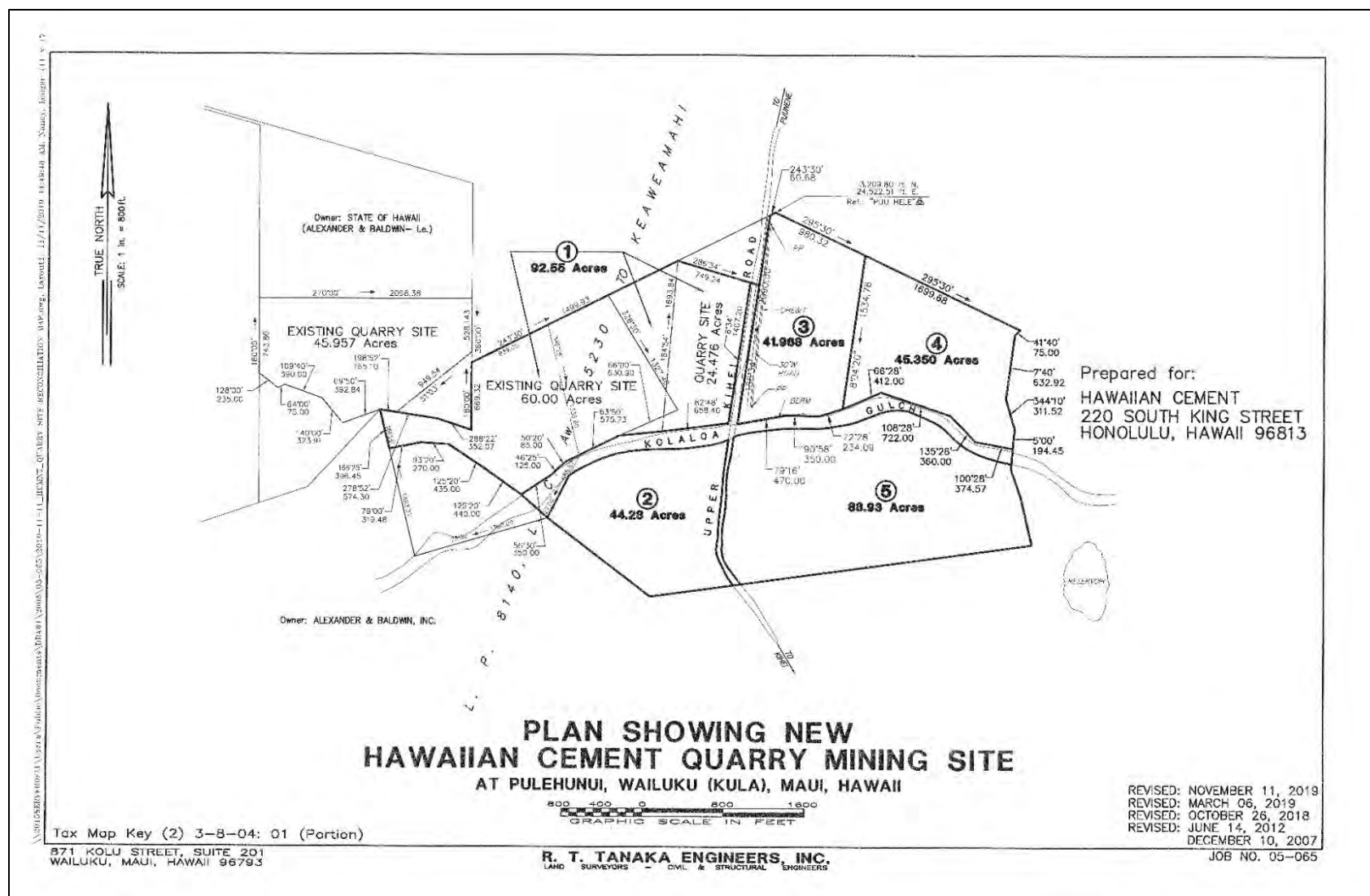
Figure 4. Hawaiian Cement Quarry Mining Site plan showing the location of Increment 4 (R.T. Tanaka Engineers Inc. 2019)
